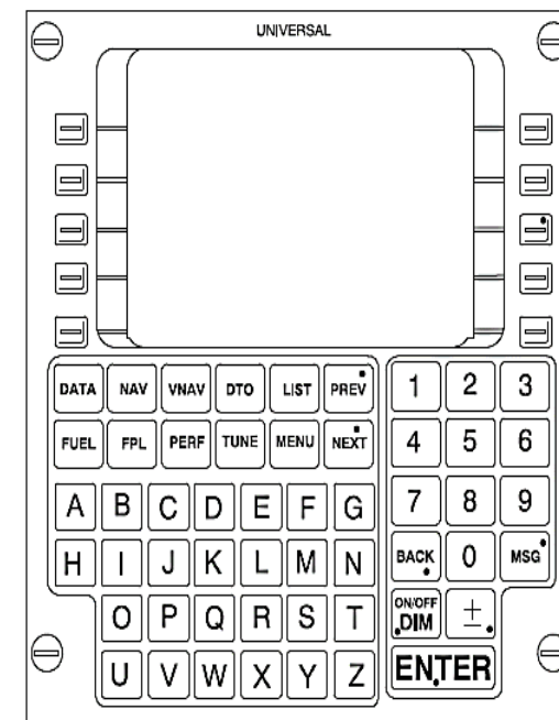
Figure - UNS-1C/1E/1EW FMS
