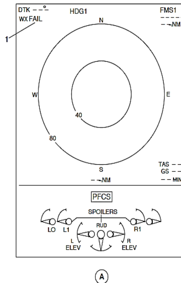
Figure 34- 109 WEATHER RADAR FAIL ANNUNCIATION
