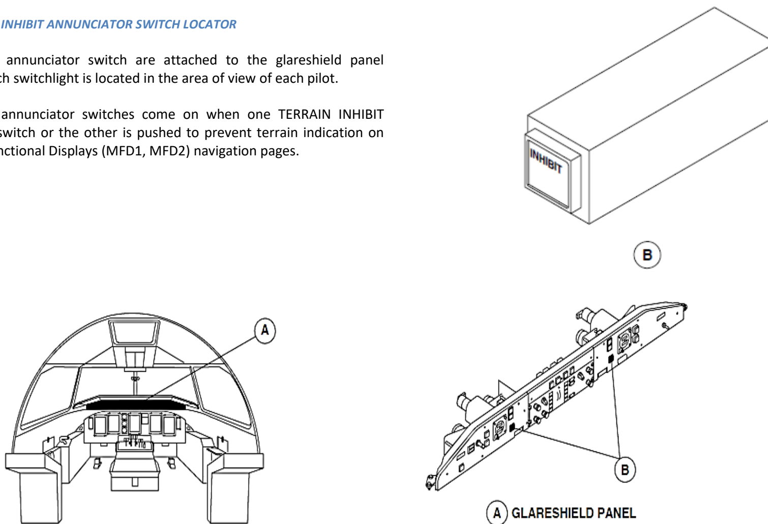
Figure 34- 144 INHIBIT ANNUNCIATOR SWITCH LOCATOR
