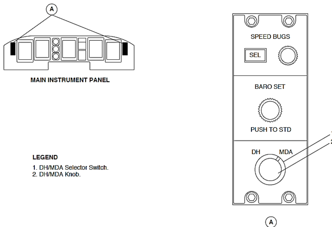
Figure 34- 28 ICP MDA SELECTION
