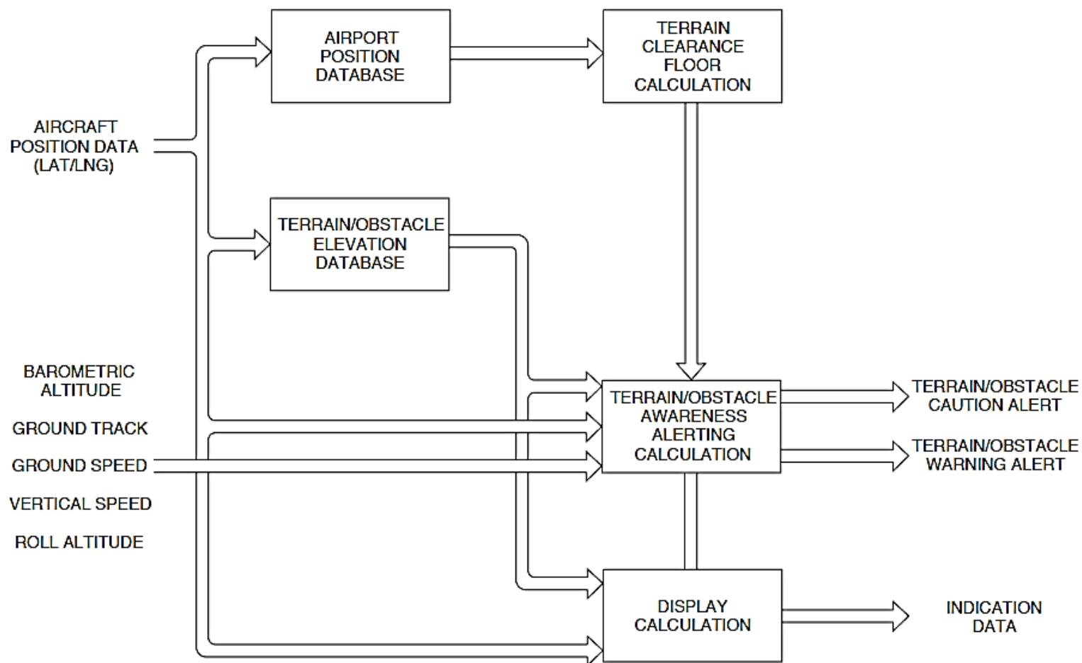
Figure 34- 135 TERRAIN ALERTING CALCULATION
