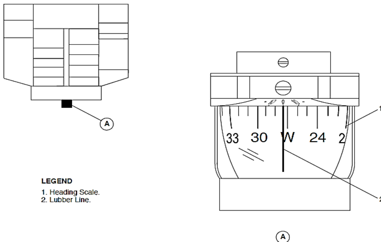
Figure 34- 97 STANDBY COMPASS
