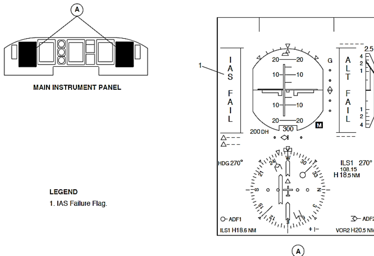
Figure 34- 18 PFD INDICATED AIR SPEED FAILURE FLAG
