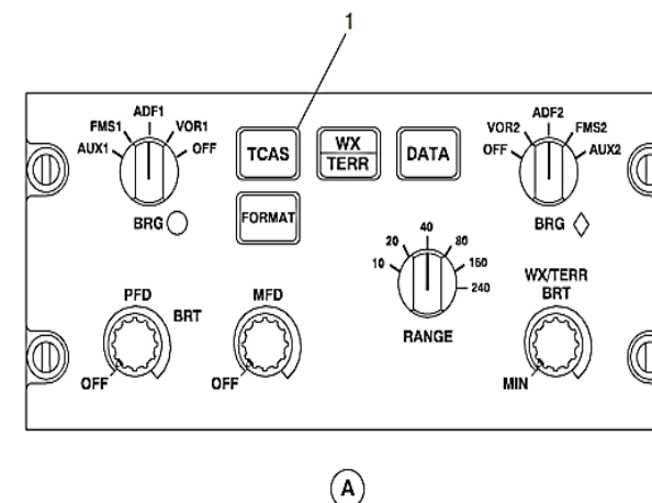
Figure 34- 168 EFCP, TCAS POP-UP OR CONTINUOUS INDICATION SELECTION
