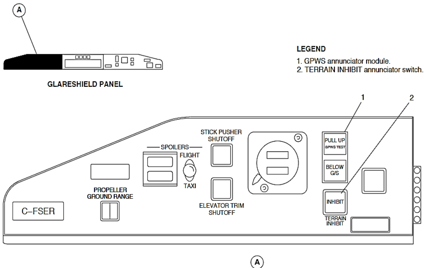
Figure 34- 146 PULL UP, BELOW G/S AND INHIBIT ANNUNCIATOR SWITCHES
