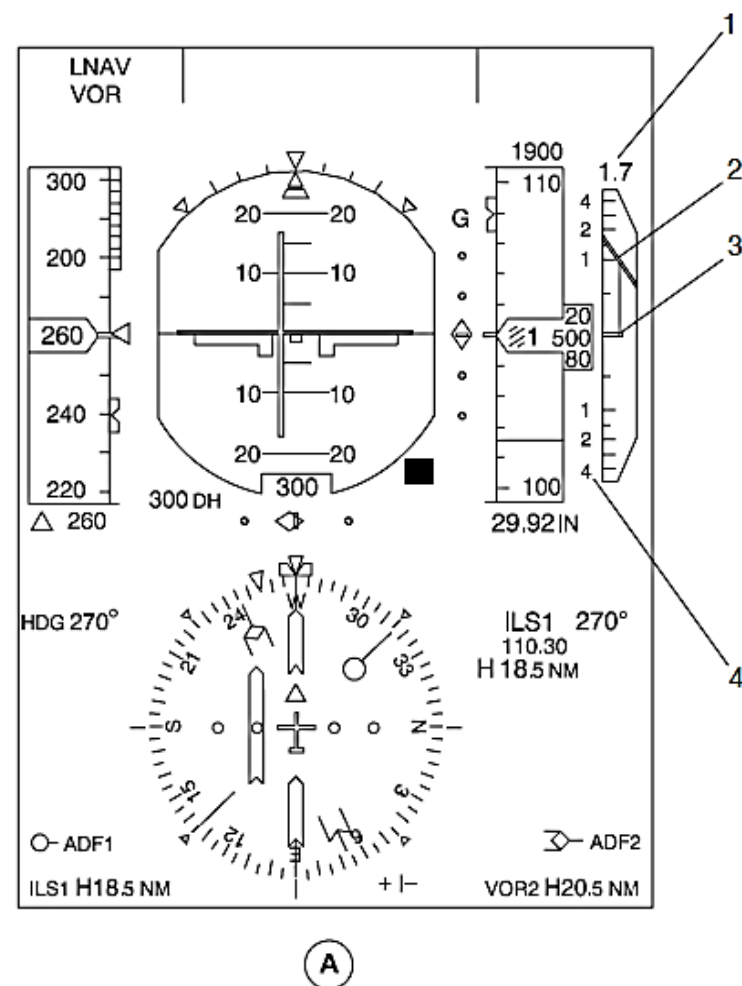
Figure 34- 71 PFD, INERTIAL VERTICAL SPEED INDICATOR INDICATIONS
