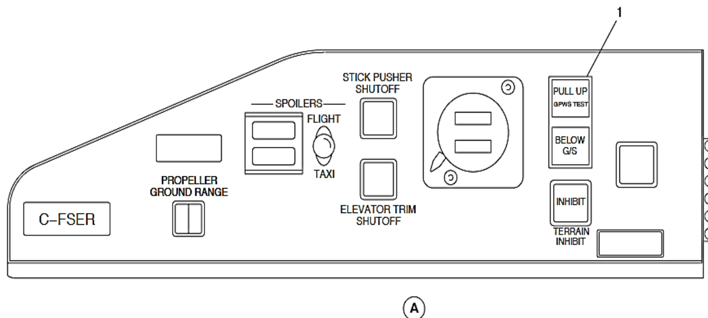
Figure 34- 153 EGPWS TEST SELECTION
