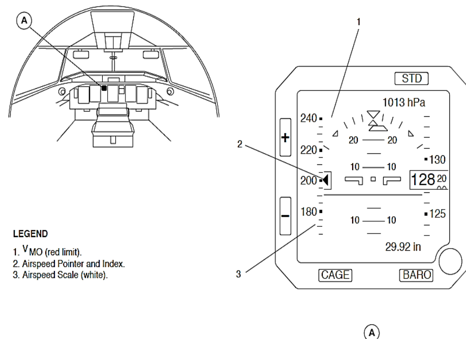
Figure 34- 52 INTEGRATED STANDBY INSTRUMENT (ISI) AIRSPEED DISPLAY
