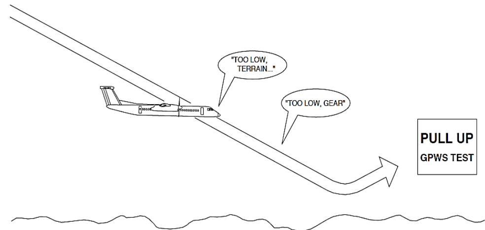
Figure 34- 119 EGPWS MODE 4A, INSUFFICIENT TERRAIN CLEARANCE INDICATIONS
