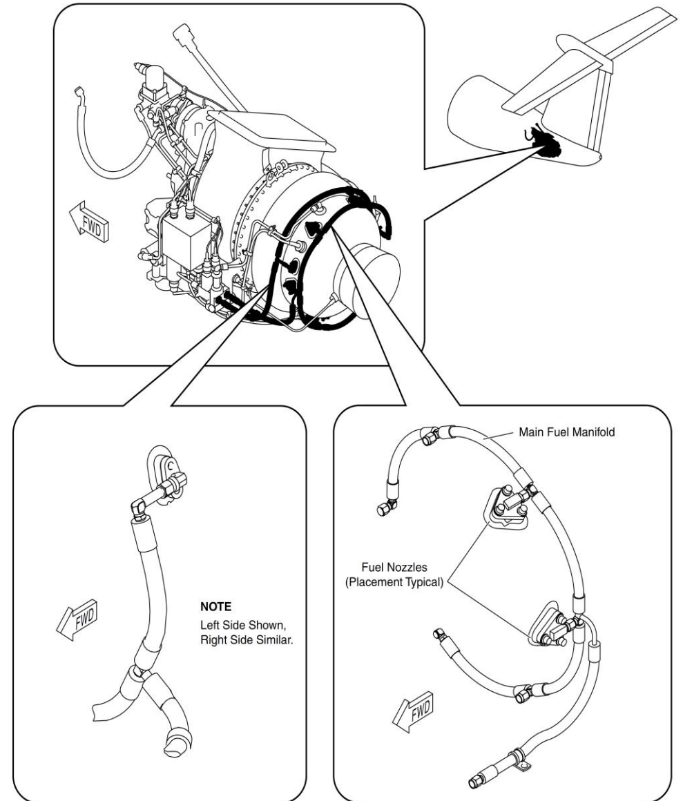
Figure 49-19 Start and Main Fuel Manifolds and Nozzles Locator
