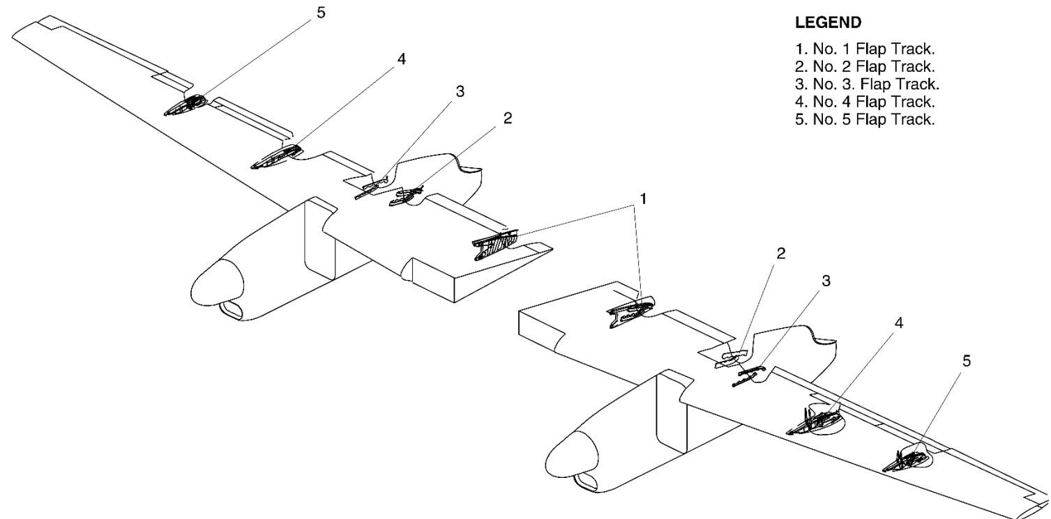
Figure 57-30 Flap Tracks - Location
