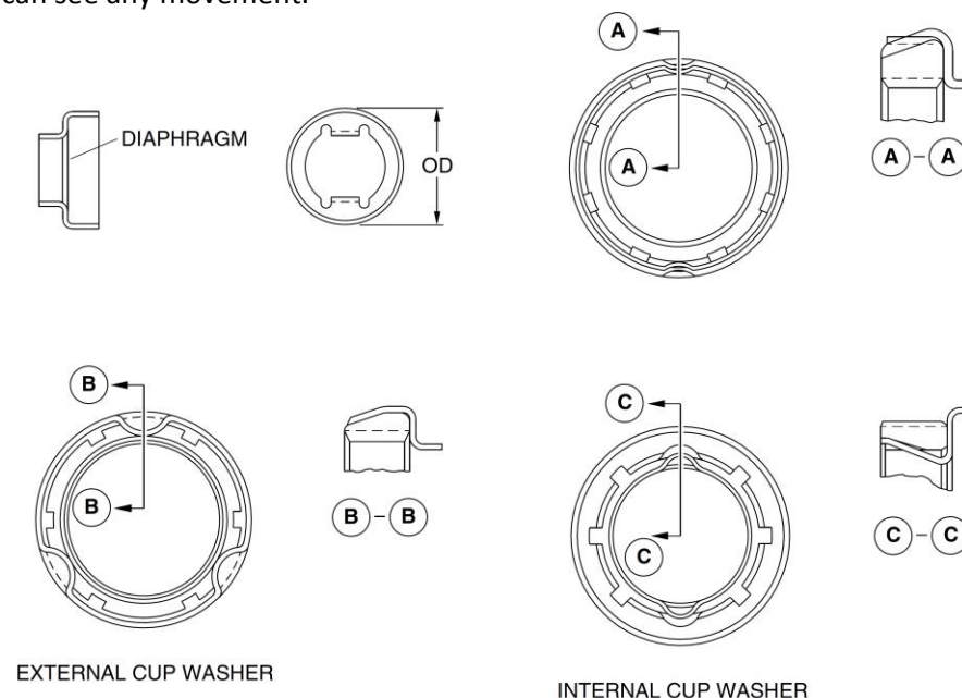
Figure 70-8 Cupwashers – Removal/Installation
