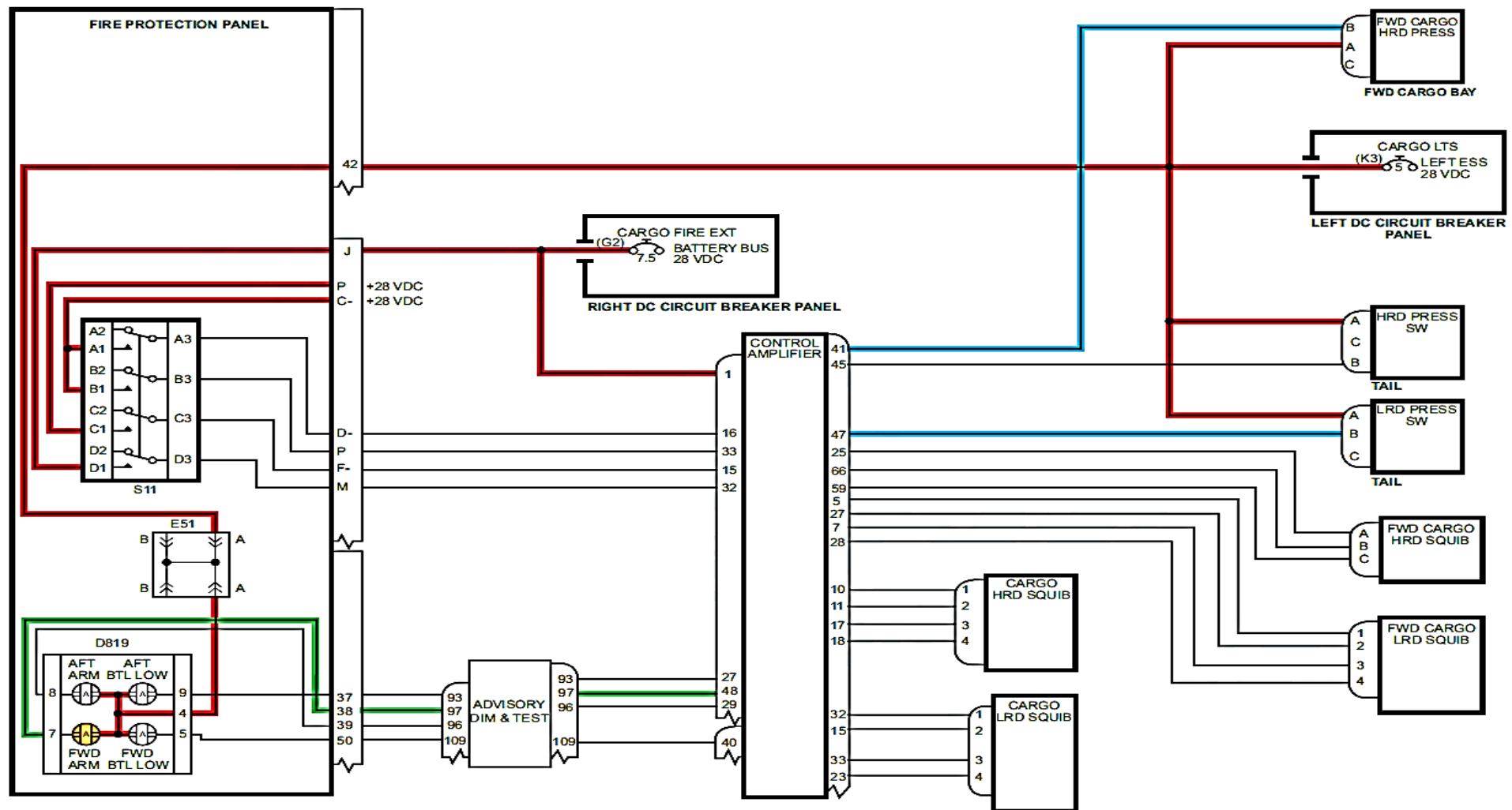
FIGURE - FORWARD BAGGAGE COMPARTMENT FIRE DETECTED
