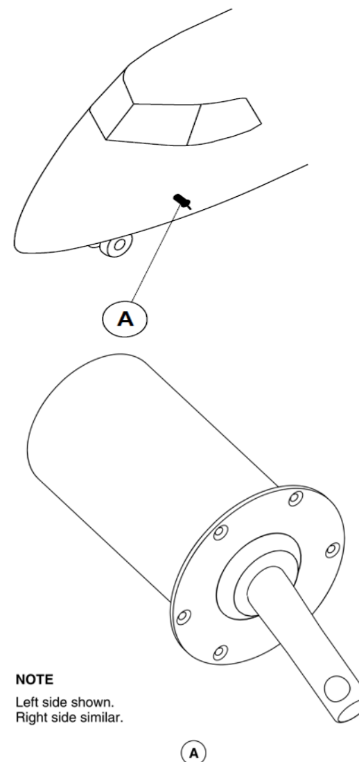
Figure 30-2 Ice detector probe – Locations
