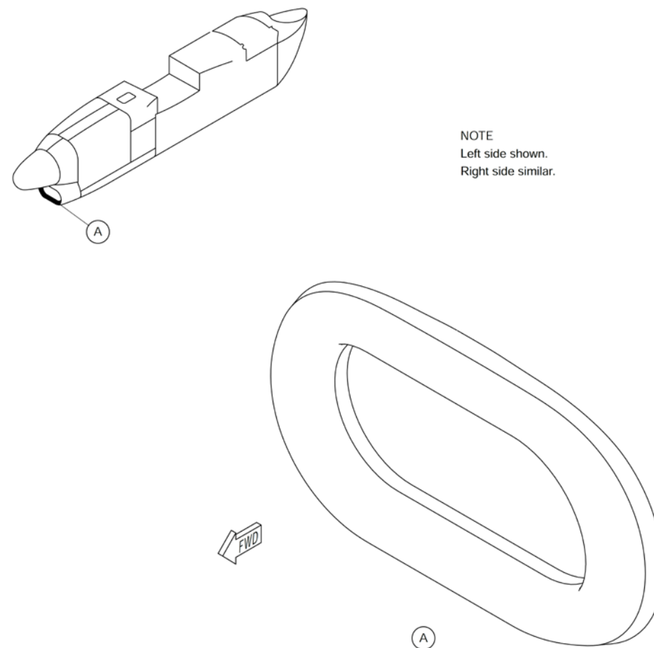
Figure 30-22 Nacelle - De-Ice Boots and Hoses
