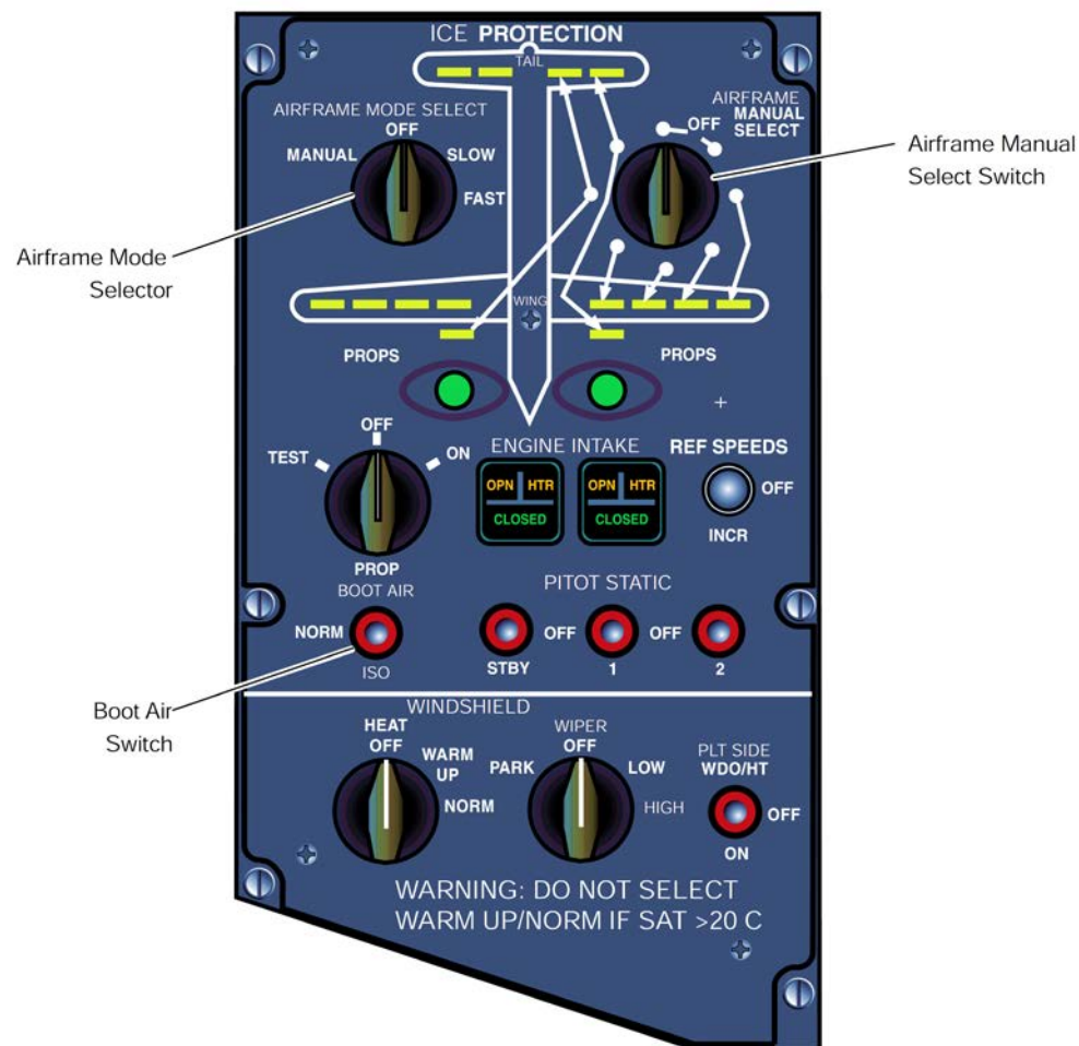
Figure 30-27 Airframe Deice Control Panel
