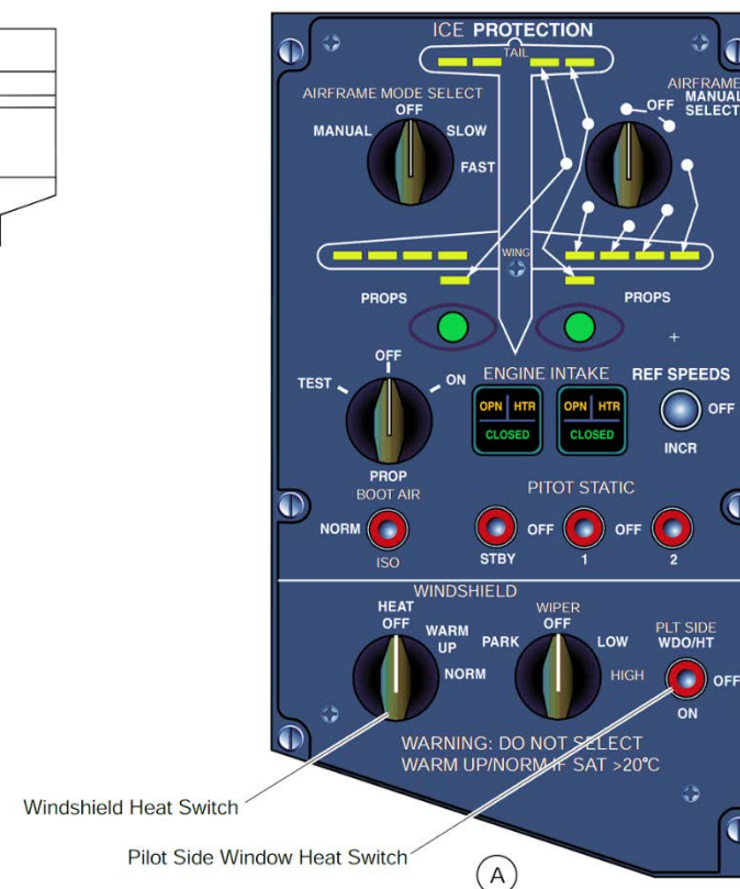
Figure 30-47 Windshield Control Panel – Location
