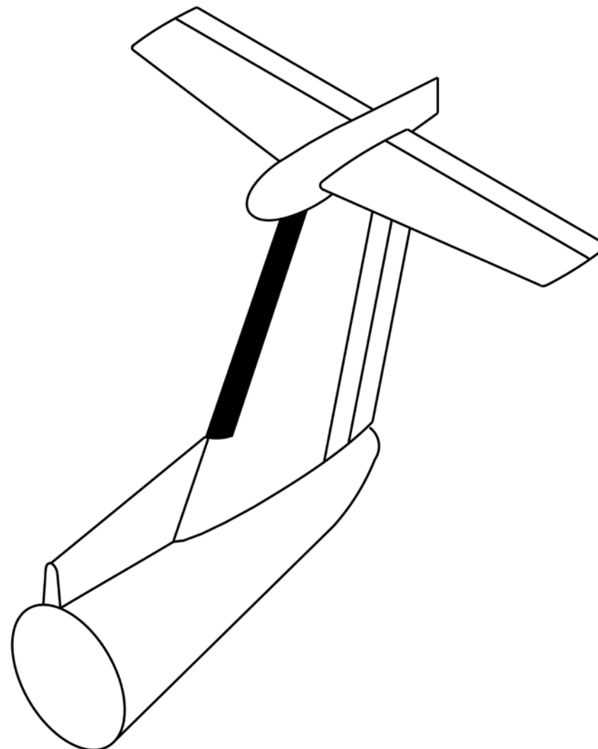
Figure 30-25 Vertical Stabilizer - De-Ice Boots and Hoses
