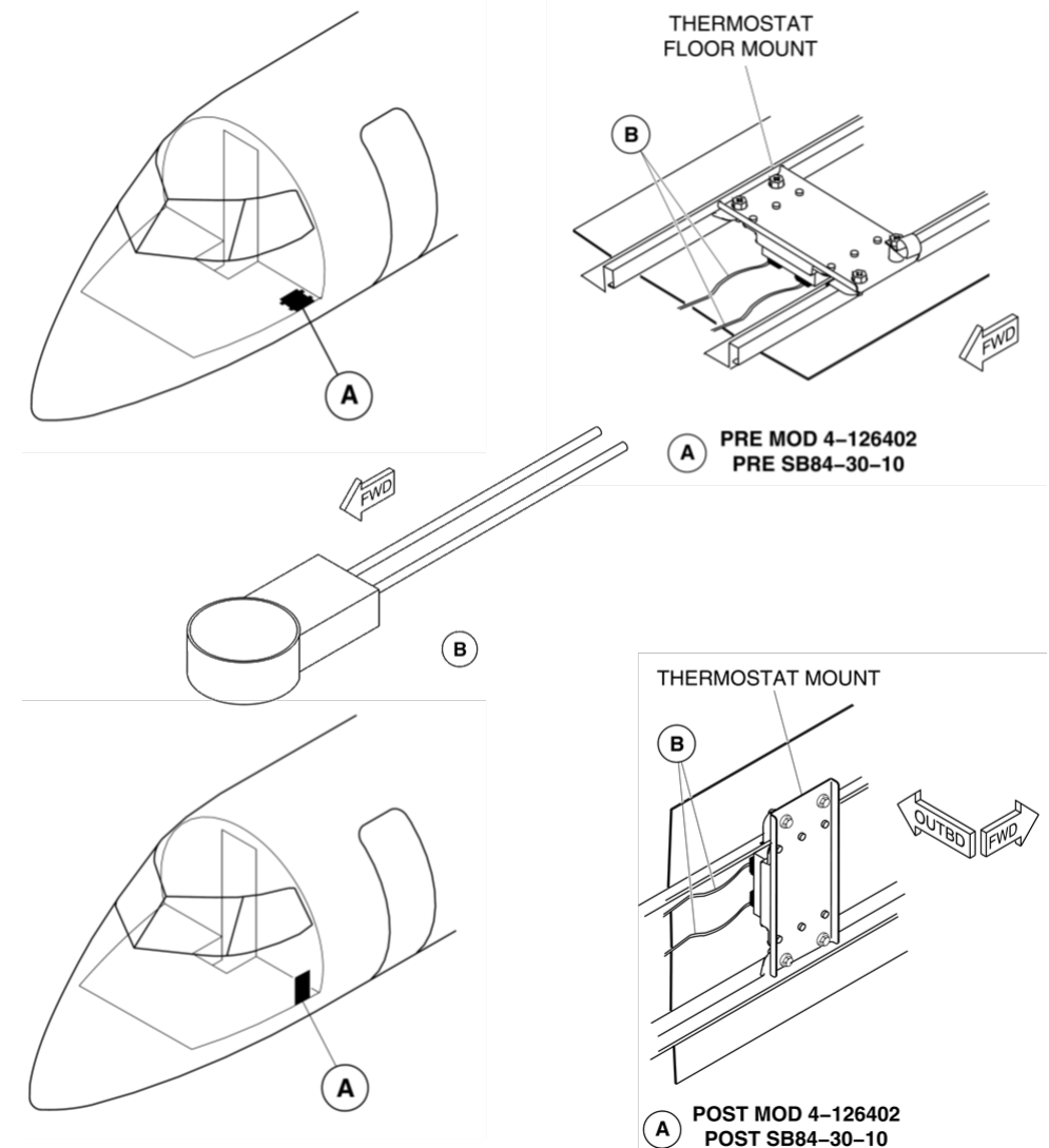
Figure 30-33 Thermostats – Location
