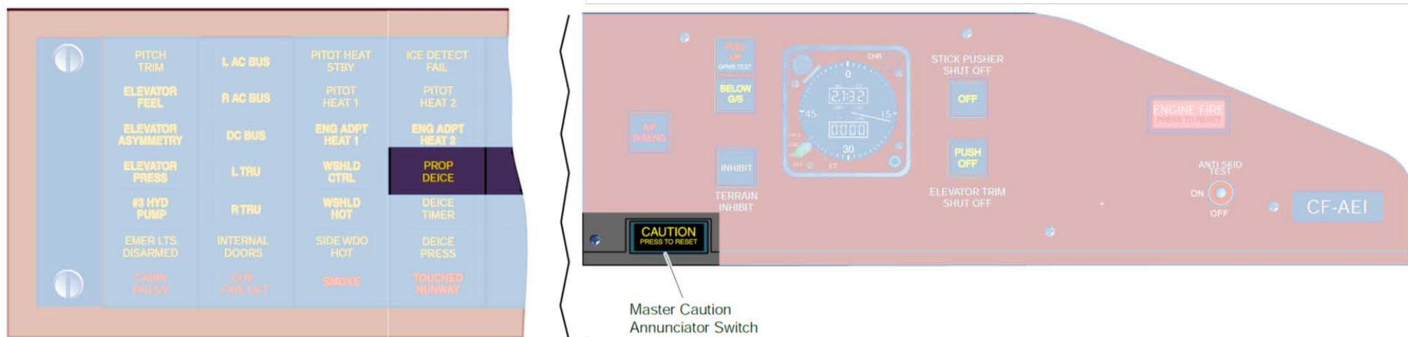
Figure 30-72 Cautions - Propellers
