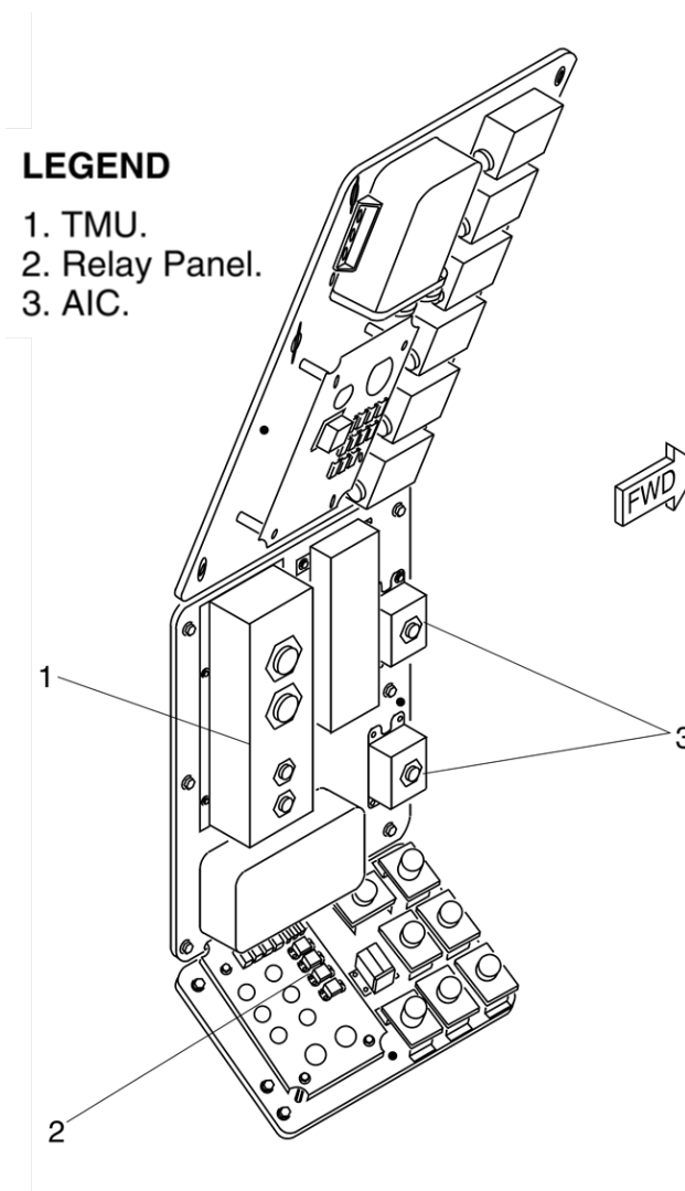
Figure 30-48 Relay Panel – Location
