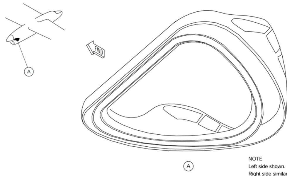
Figure 30-31 Engine Air Intake – Location
