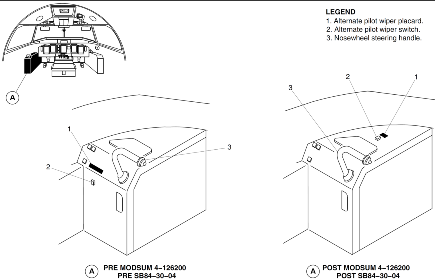
Figure 30-59 Alternate Pilot Switch – Location
