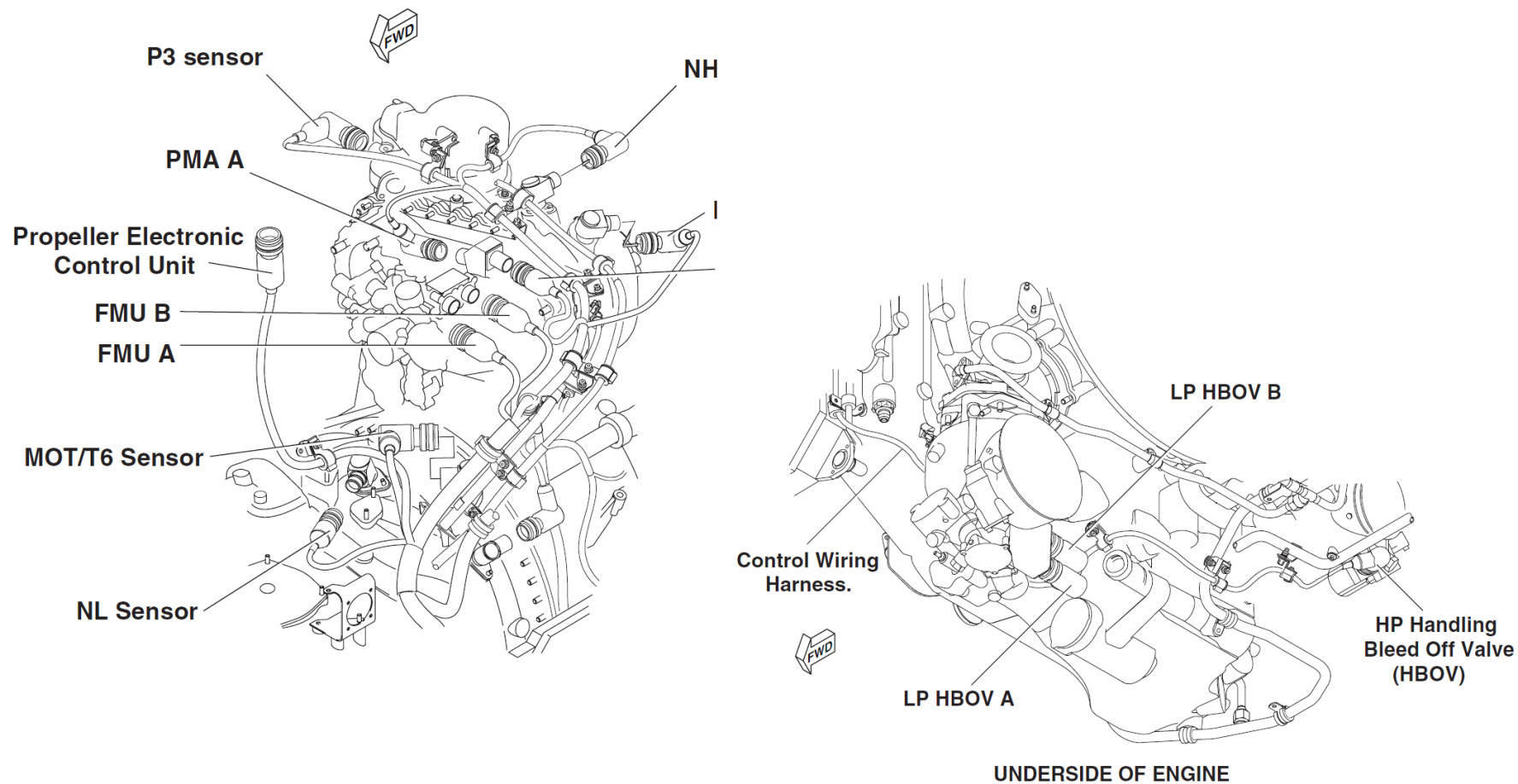
Figure 73-19 Electrical Wiring – Fuel Control Harness (2 of 2)
