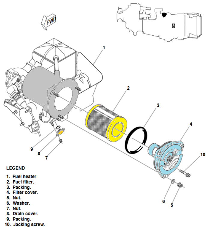
Figure 73-11 Fuel Filter
