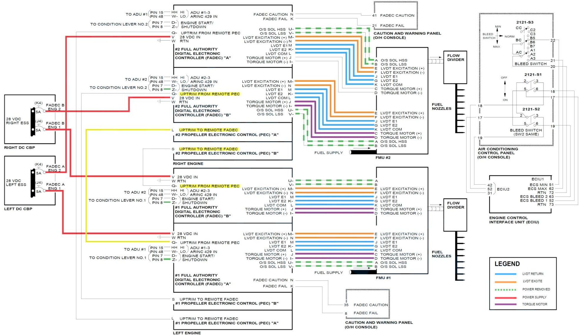
Figure 73-24 FADEC Control
