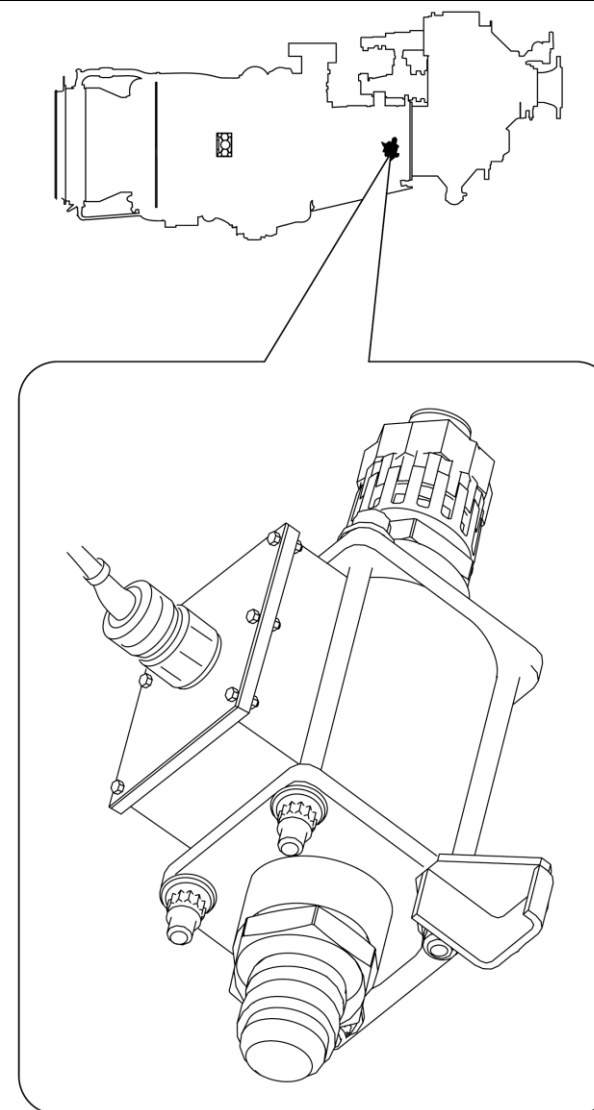
Figure 73-7 Fuel Flowmeter
