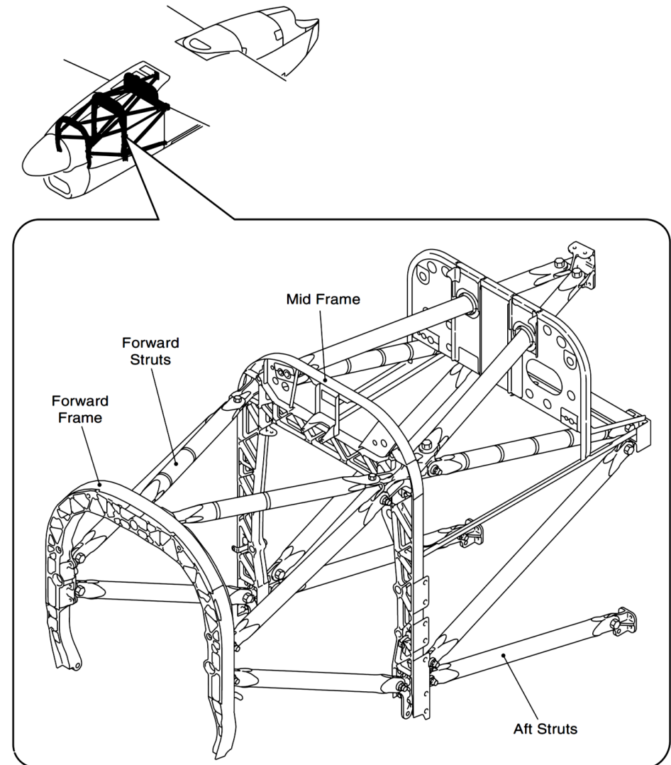
Figure 54-7 Nacelle Support Frames and Struts
