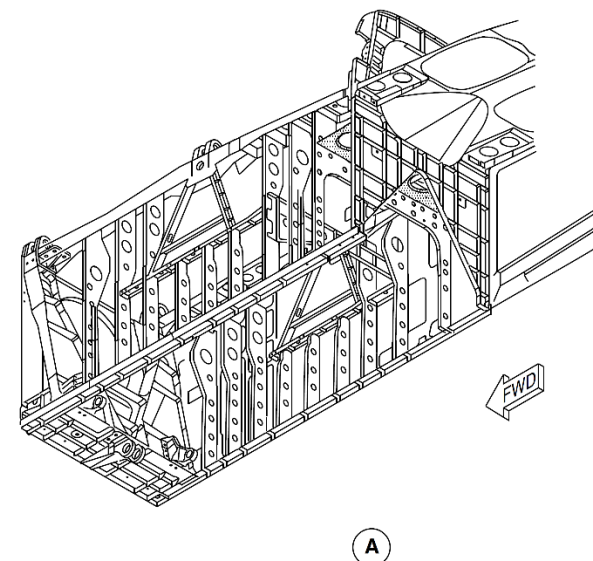
Figure 54-4 Center Nacelle - Location
