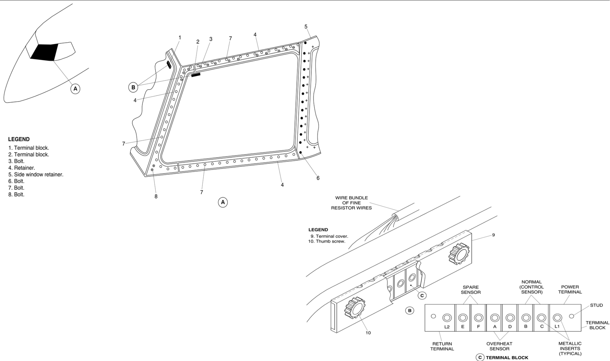
Figure 56-5 Windshield
