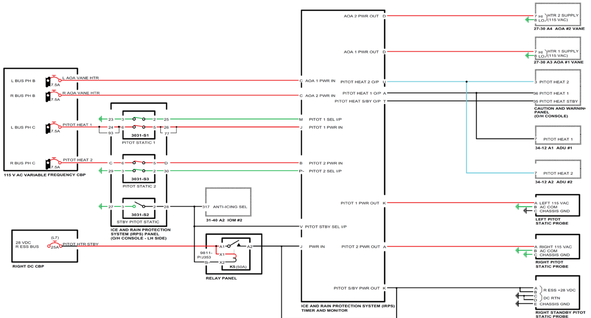
Figure 30-41 Pitot and Static Anti-Icing - Electrical Schematic
