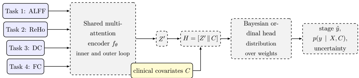
Figure 4.2: The Meta-Bayesian pipeline (design, not implemented). The four biomarkers act as meta-learning tasks; the clinical covariates are fused after the shared representation is learnt.
