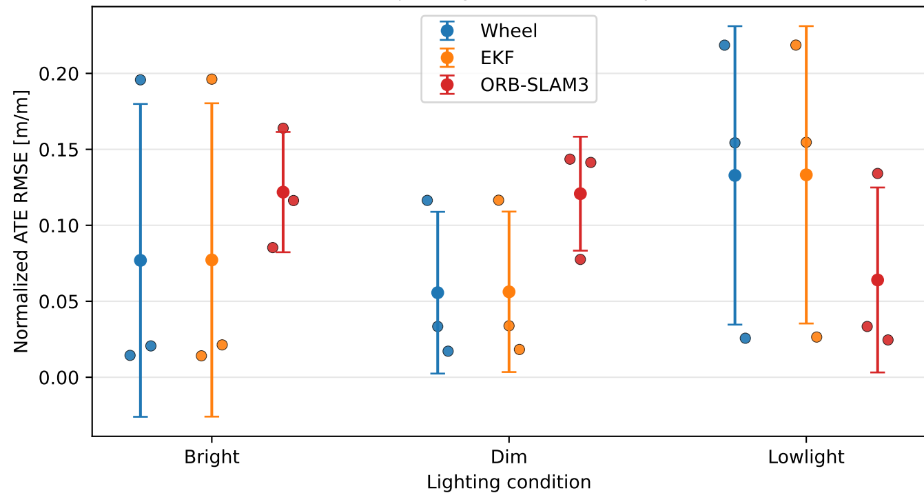
Normalized trajectory error across repeated trials
