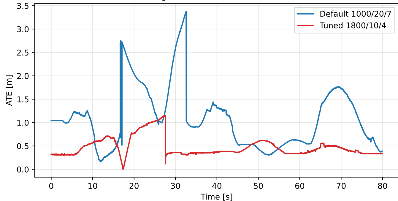
Lowlight t03 ORB-SLAM3 ablation
