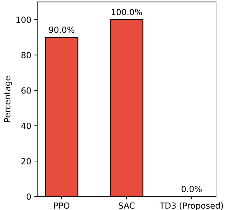
Collision Rate (%)
