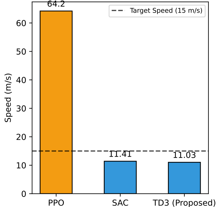
Mean Velocity (m/s)
