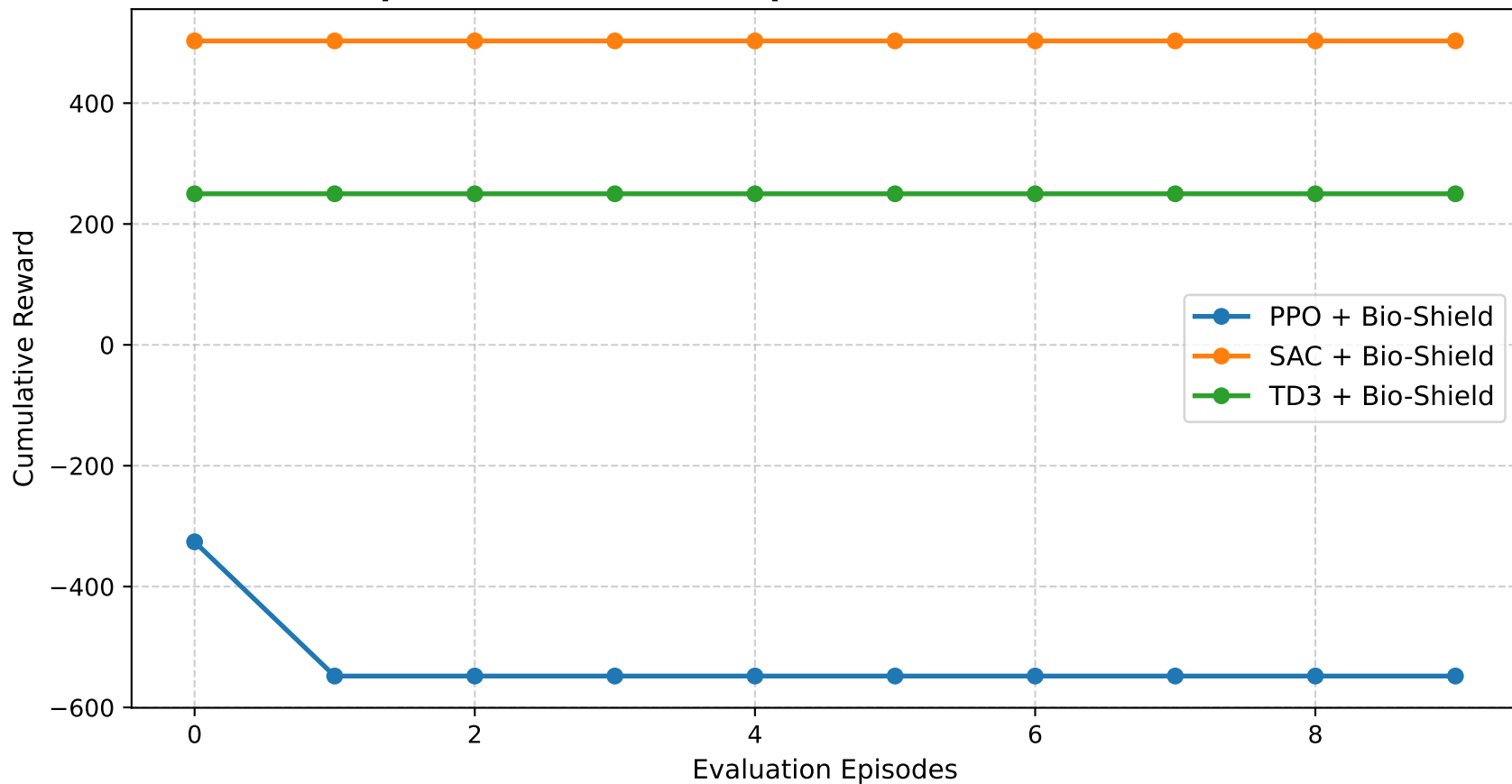
Comparative Cumulative Episode Reward (Bio-Shielded RL)
