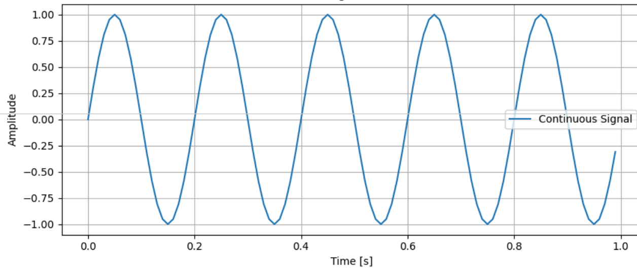
Sampling of Continuous Signal ( f_s = 100 Hz)
