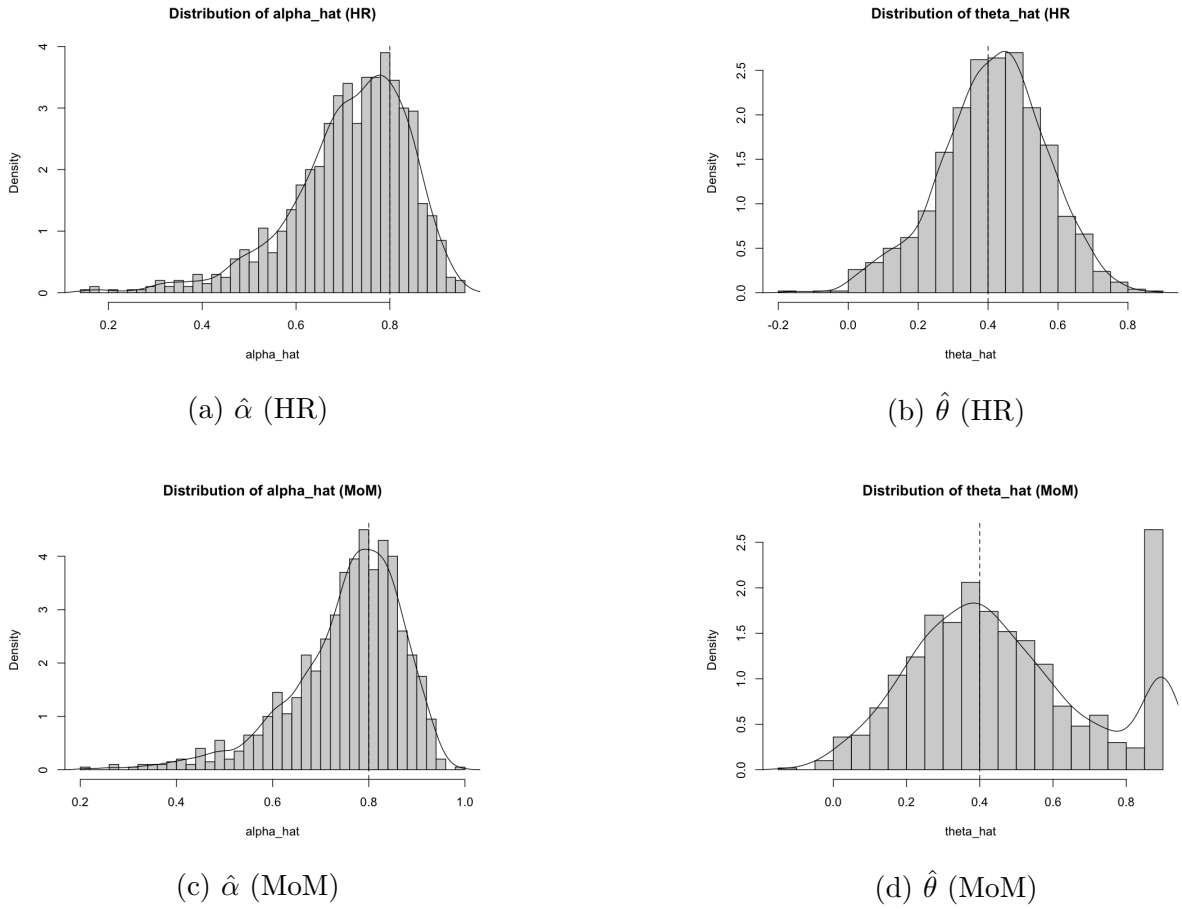
Figure 4: Distributions of parameter estimates. Dashed vertical line indicates the true parameter value.
