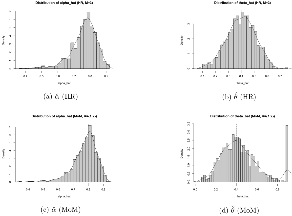
Figure 3: Distributions of parameter estimates. Dashed vertical line indicates the true parameter value.
