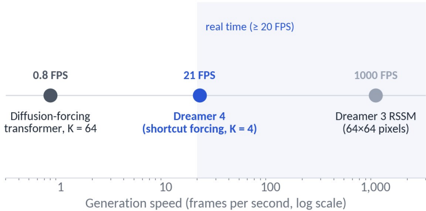
Generation speed on a log scale (paper, TalkRL): ~30× faster than diffusion forcing, ~40× slower than the RSSM.
