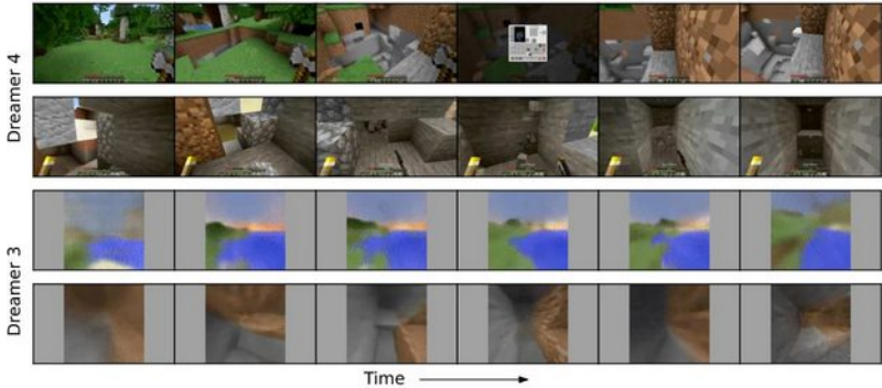
Figure 11: multi-step generations, Dreamer 4 (top) vs Dreamer 3 (bottom).
