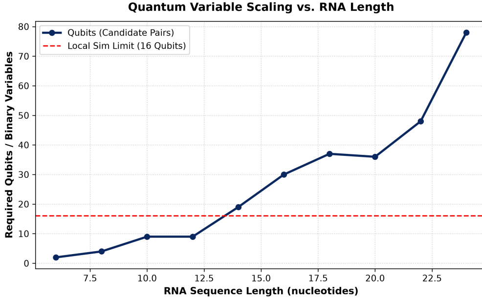
Figure 3: Empirically measured qubit count (candidate-pair count) versus RNA sequence length on random sequences. The dashed line marks the practical local statevector-simulation limit of about 16 qubits; the curve crosses it between 12 and 14 nucleotides. The non-monotonic behavior around 20 nt reflects the random sequence composition at each length.
