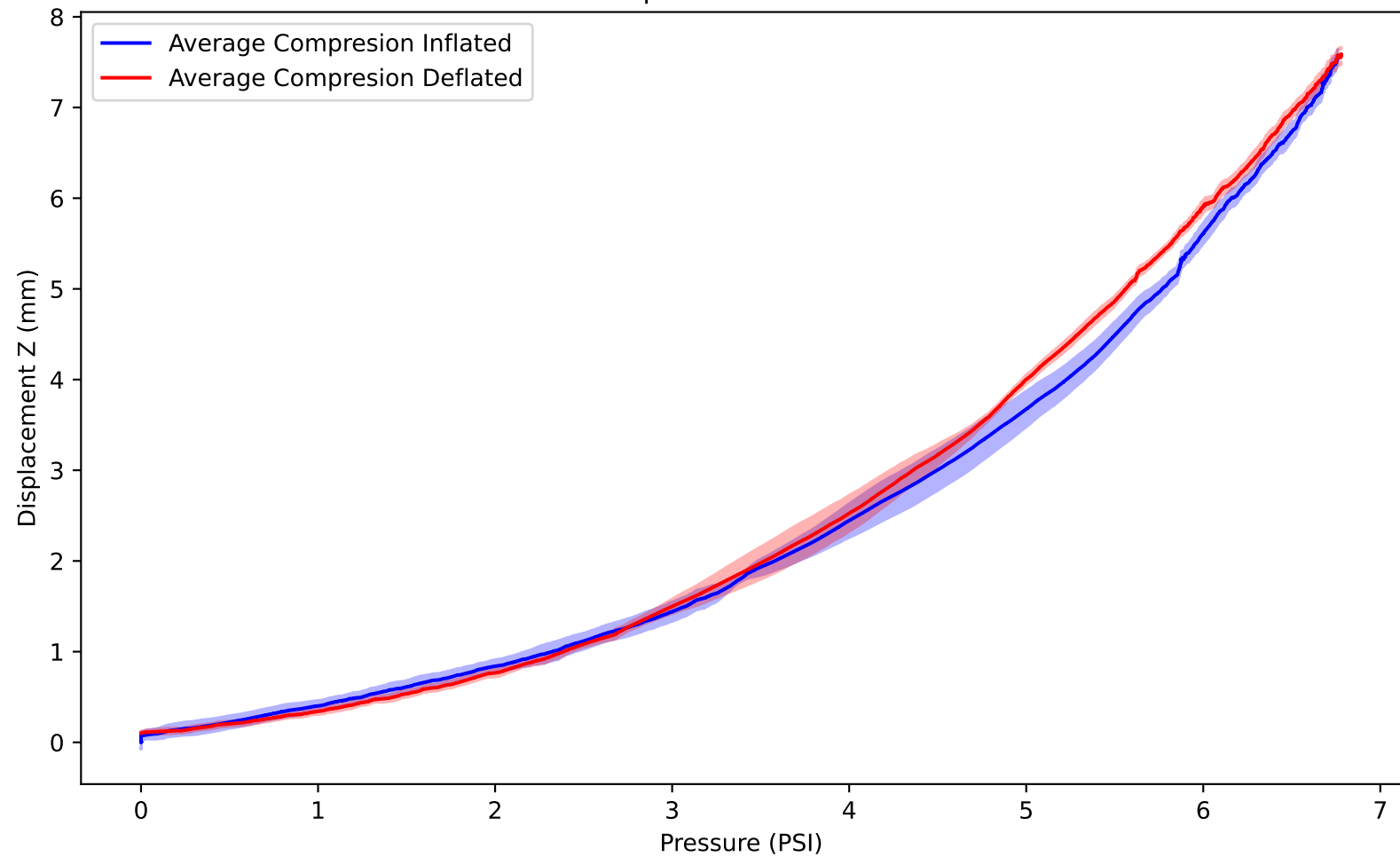
Pressure vs Displacement Z - Robot Uniaxial
