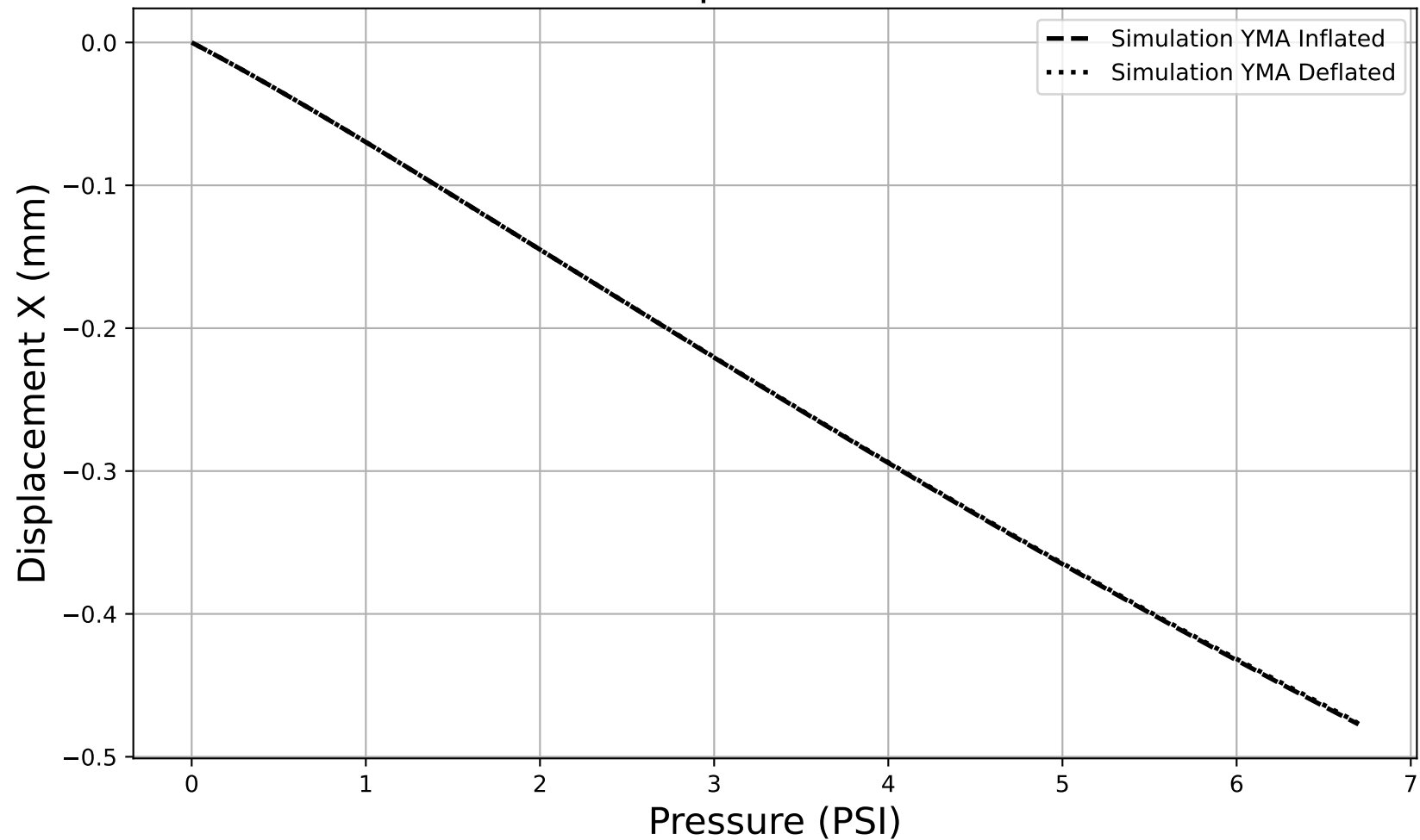
Pressure vs Displacement X - Uniaxial
