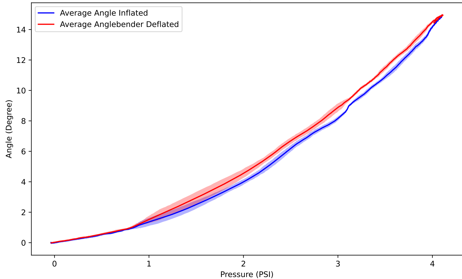
Pressure vs Angle - Robot Tilt
