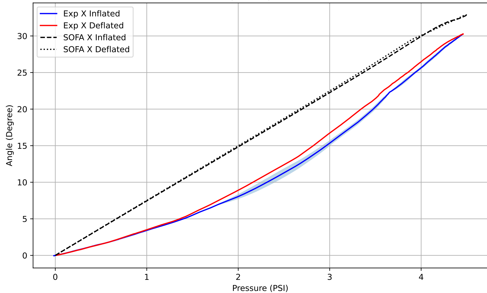
Pressure vs Angle - Experimental vs SOFA
