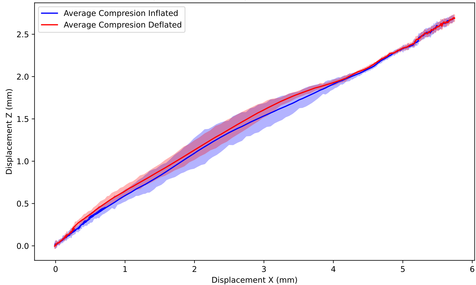
Displacement Z vs Displacement X - Robot Shear
