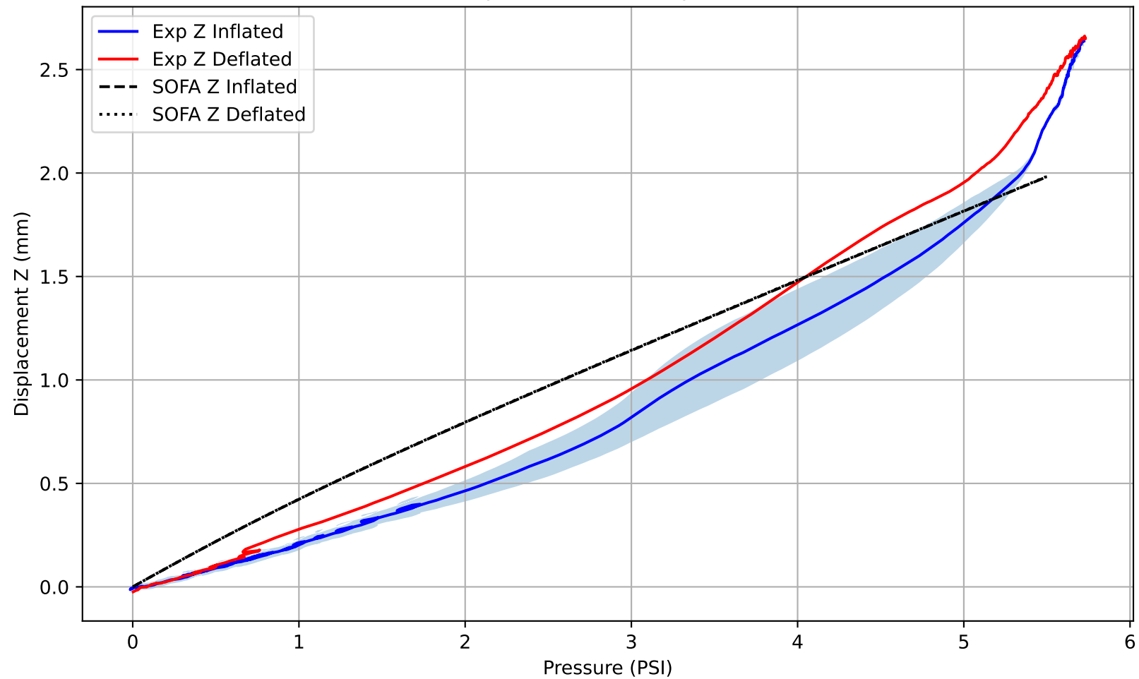
Pressure vs Displacement Z - Experimental vs SOFA
