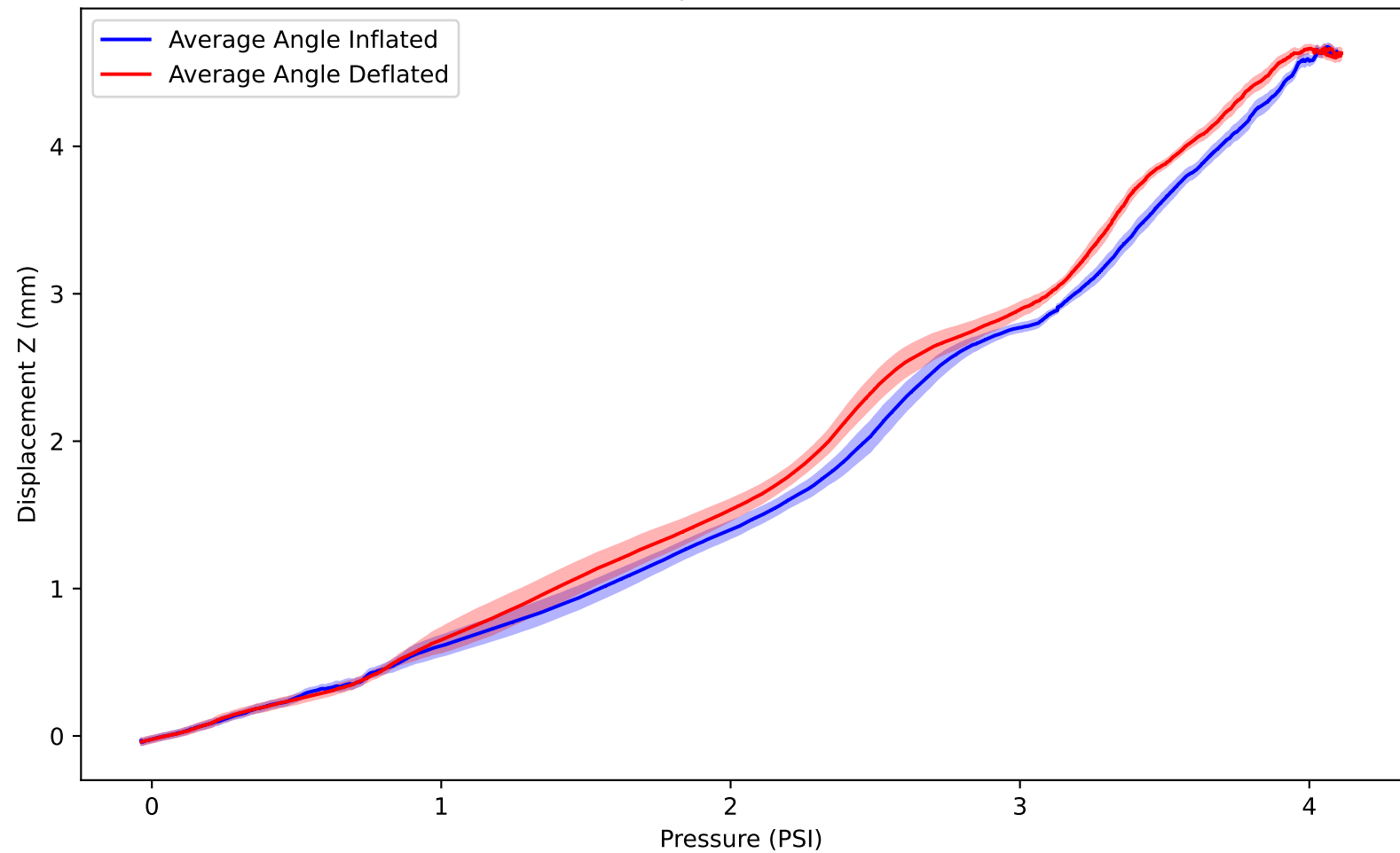
Pressure vs Displacement Z - Robot Tilt
