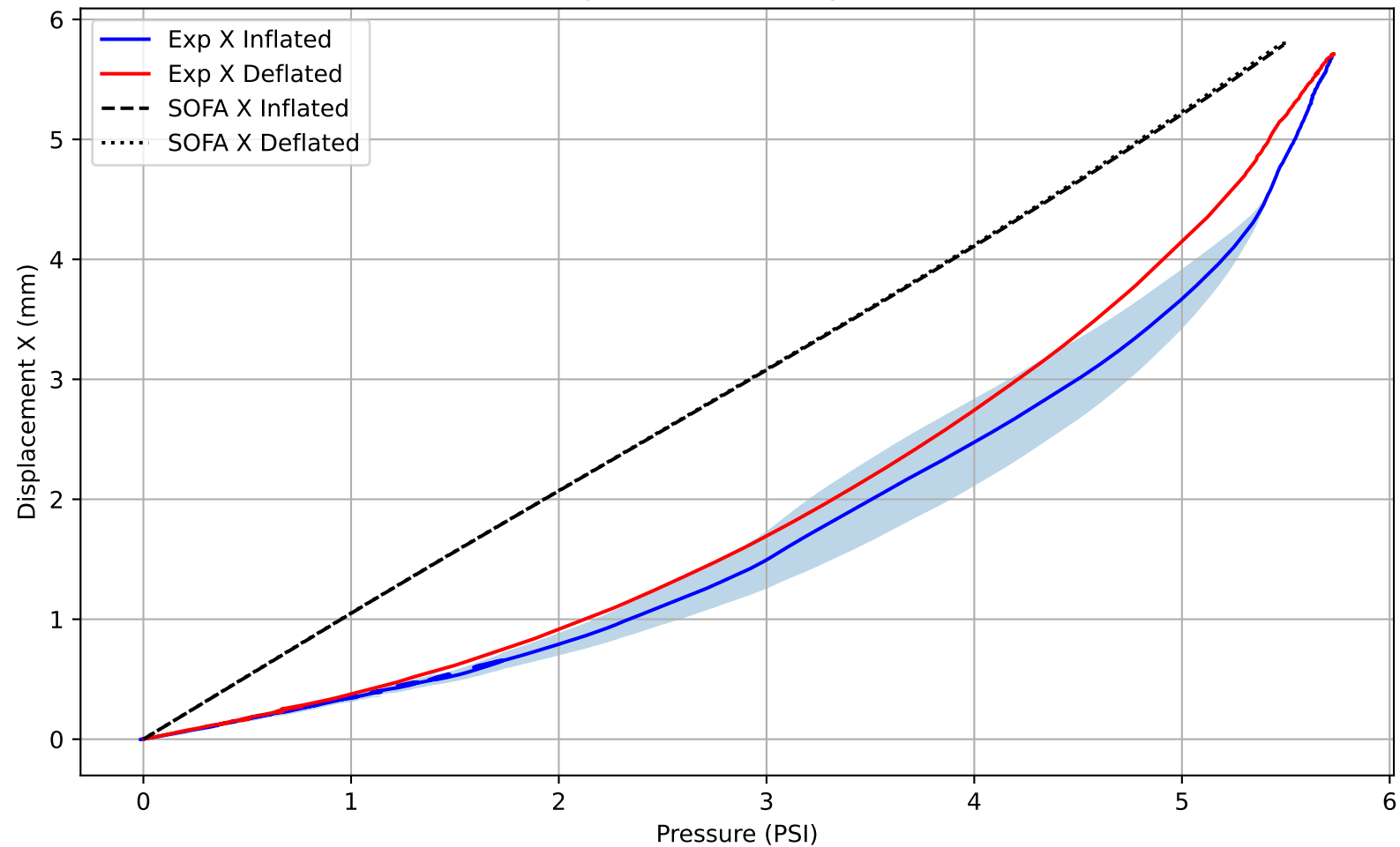
Pressure vs Displacement X - Experimental vs SOFA
