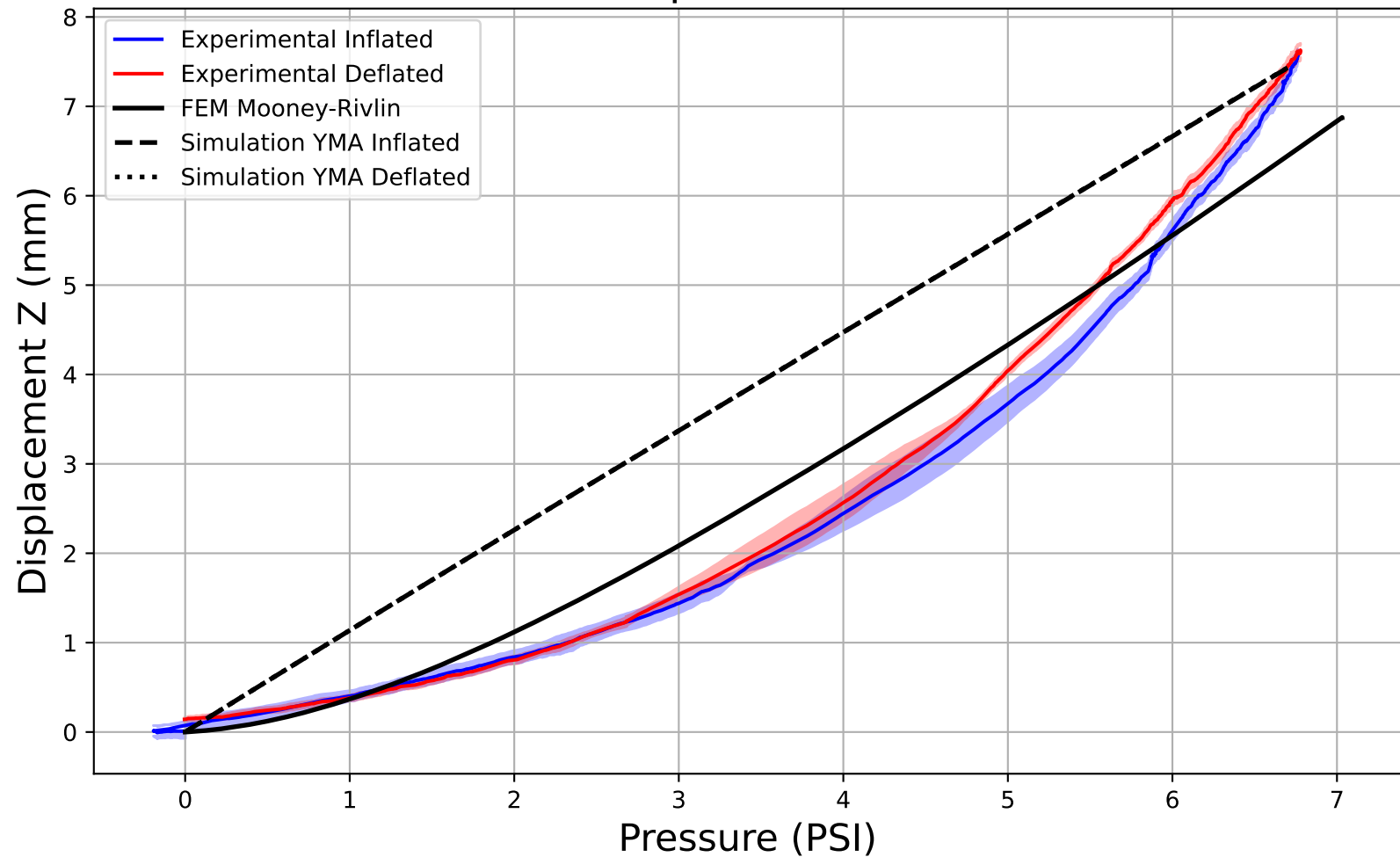
Pressure vs Displacement Z - Uniaxial
