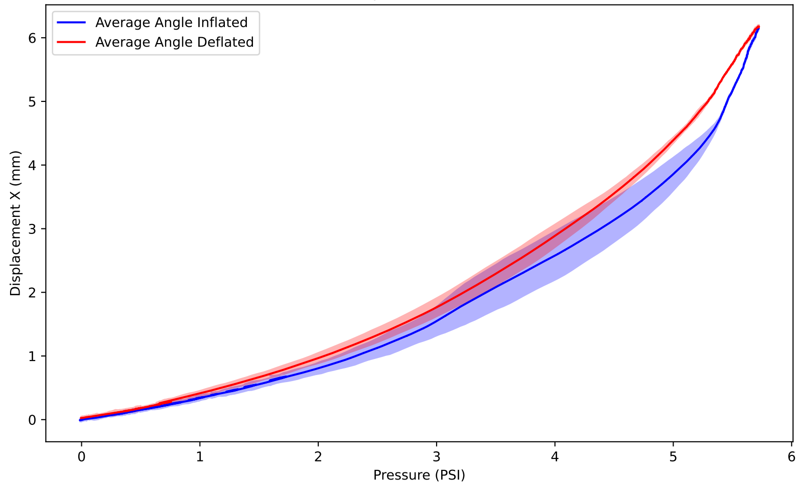
Pressure vs Displacement X - Robot Shear
