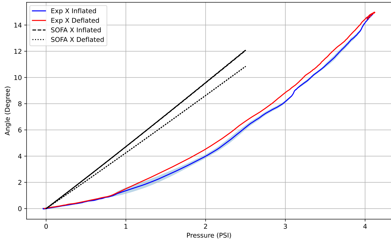
Pressure vs Angle - Experimental vs SOFA
