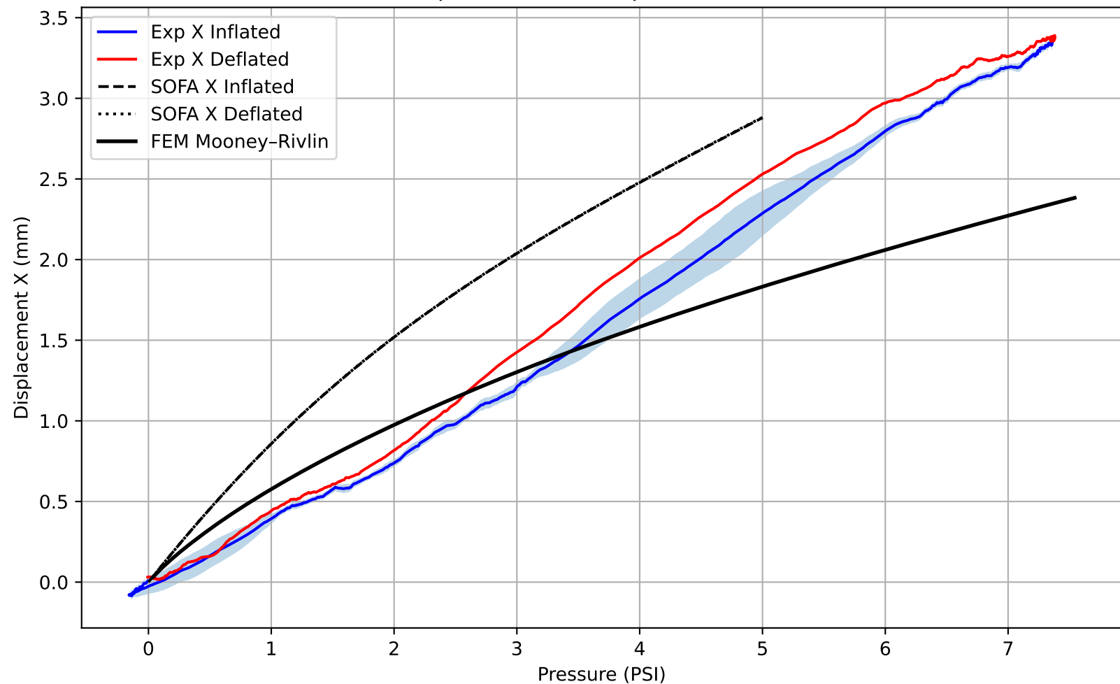
Pressure vs Displacement X - Experimental vs SOFA vs FEM
