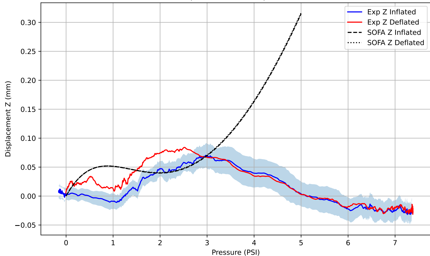
Pressure vs Displacement Z - Experimental vs SOFA
