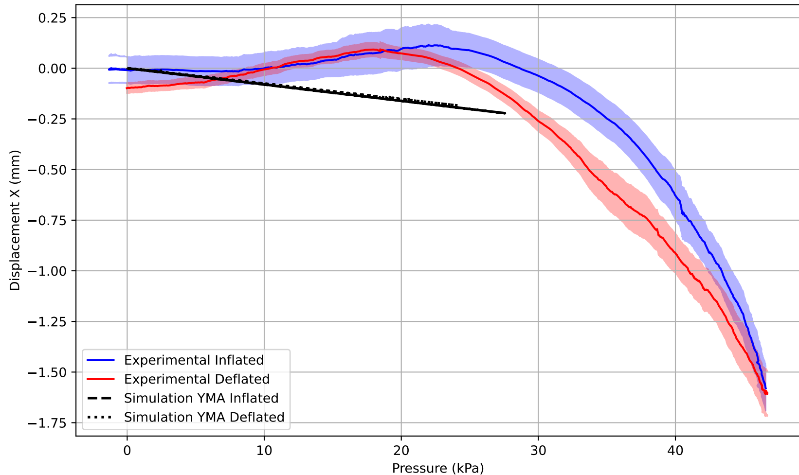
Undesired Deformation (X)
