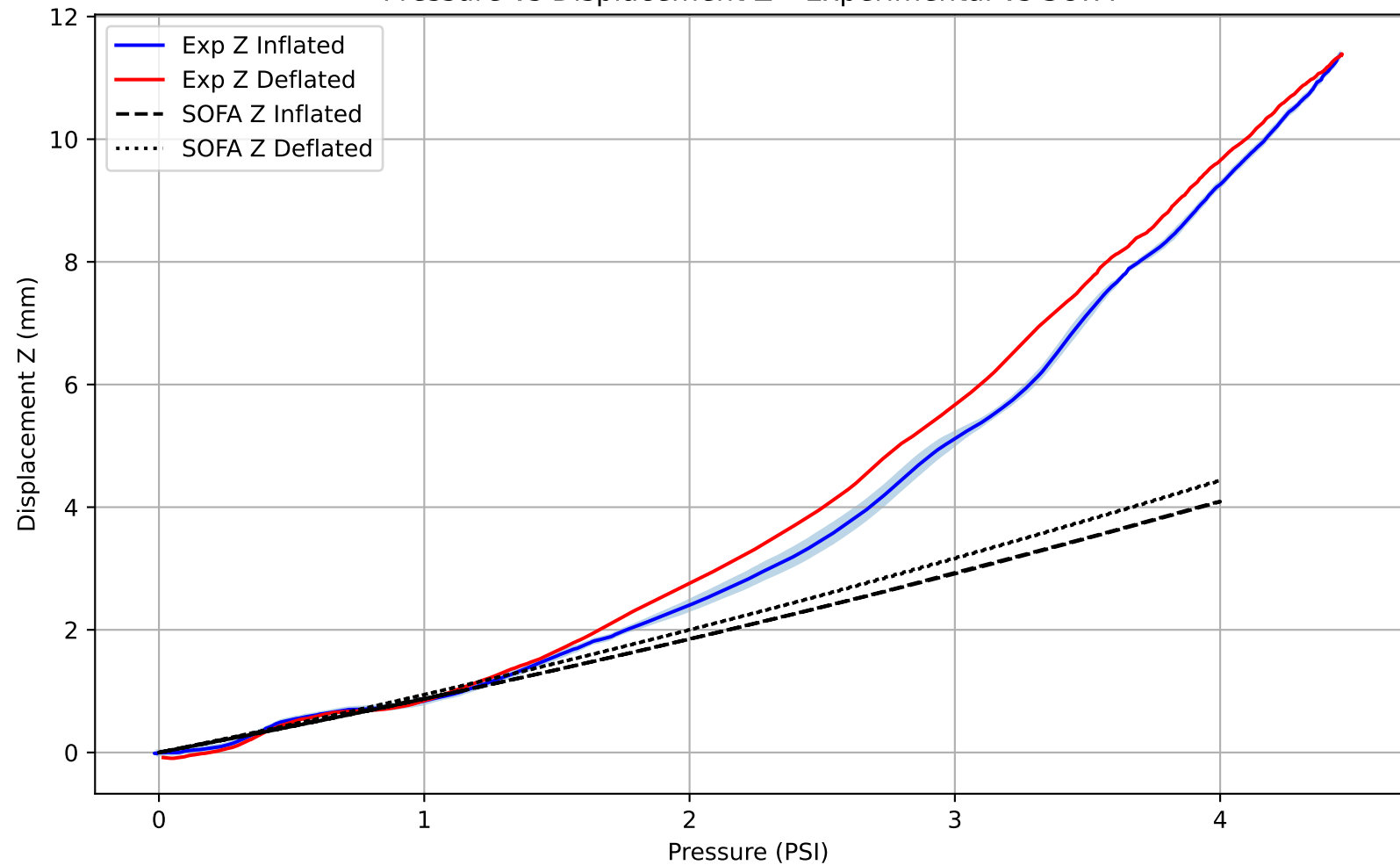
Pressure vs Displacement Z - Experimental vs SOFA
