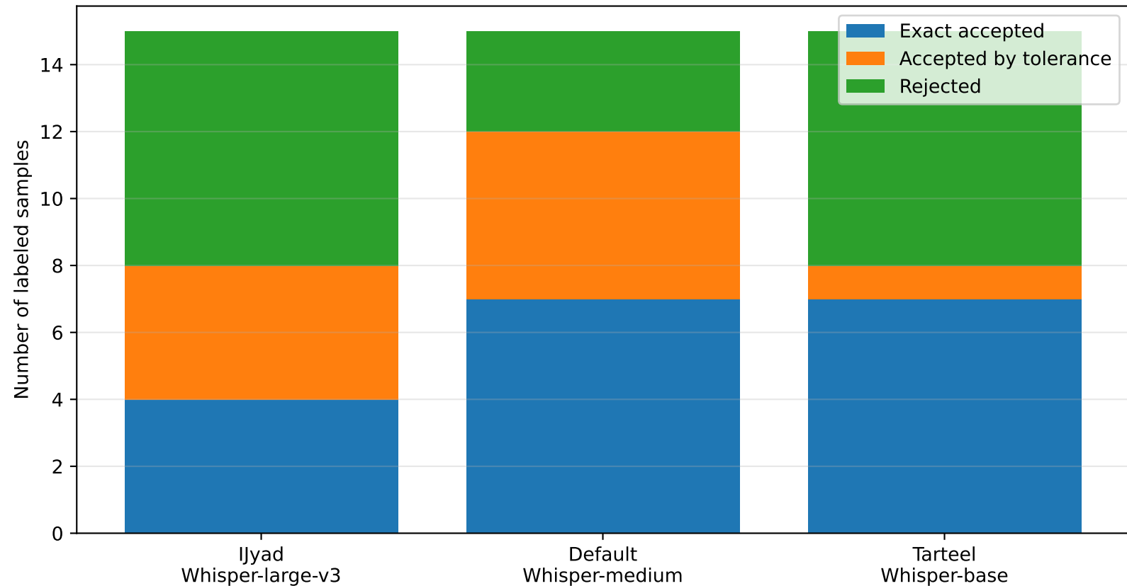
Content gate outcome breakdown by ASR model
