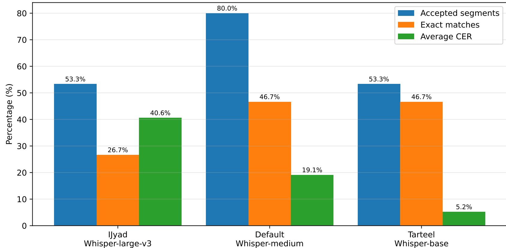
Labeled content-ASR comparison: acceptance, exactness, and CER
