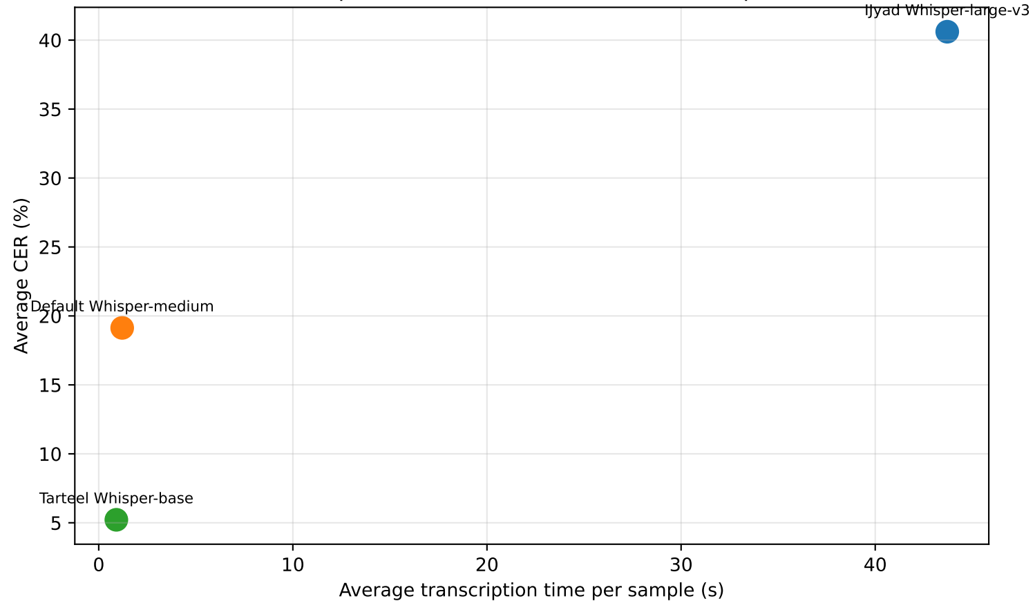
ASR speed--error trade-off on labeled samples
