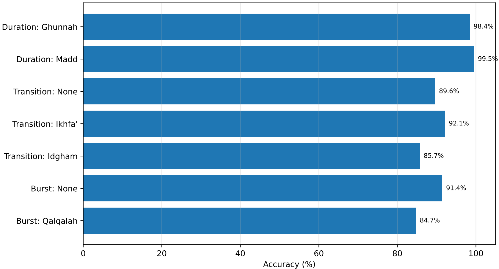
Per-class accuracy across Tajweed modules
