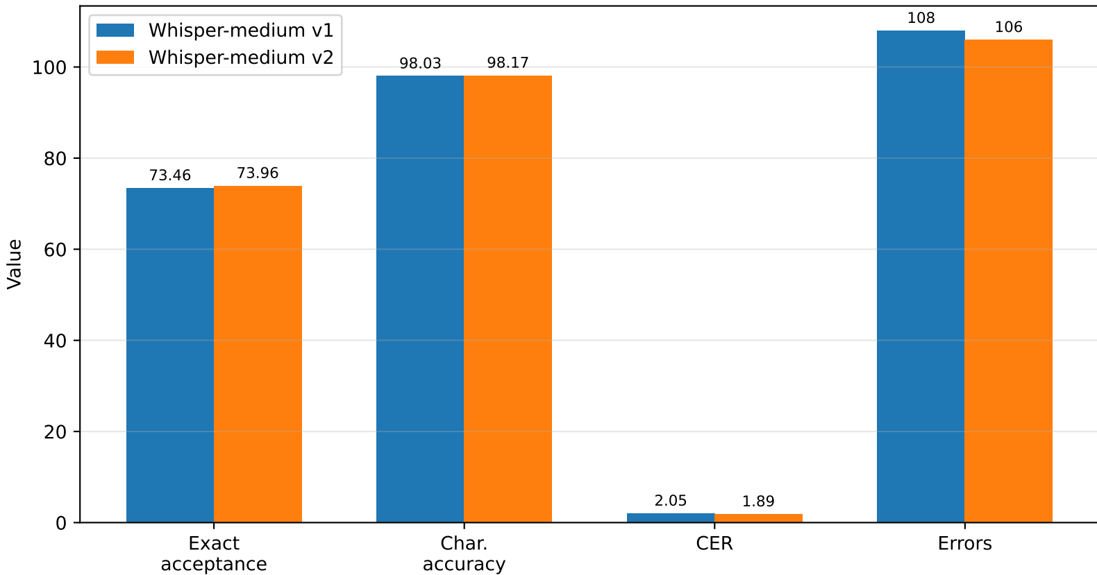
Whisper content gate ablation: v1 versus v2
