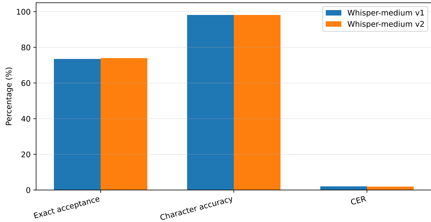
Content gate ablation: v1 versus v2
