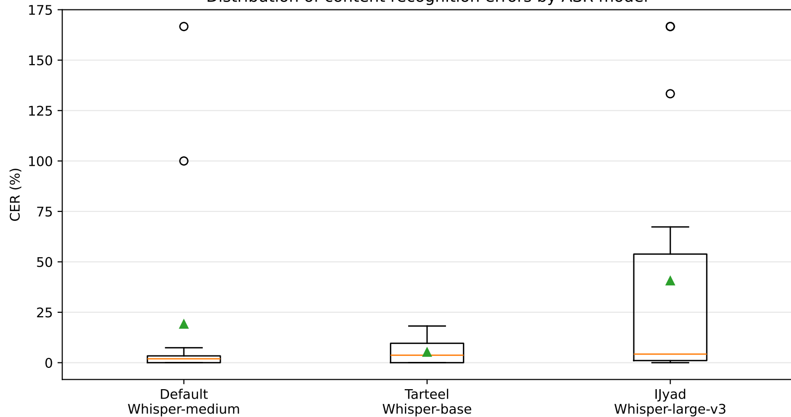
Distribution of content recognition errors by ASR model
