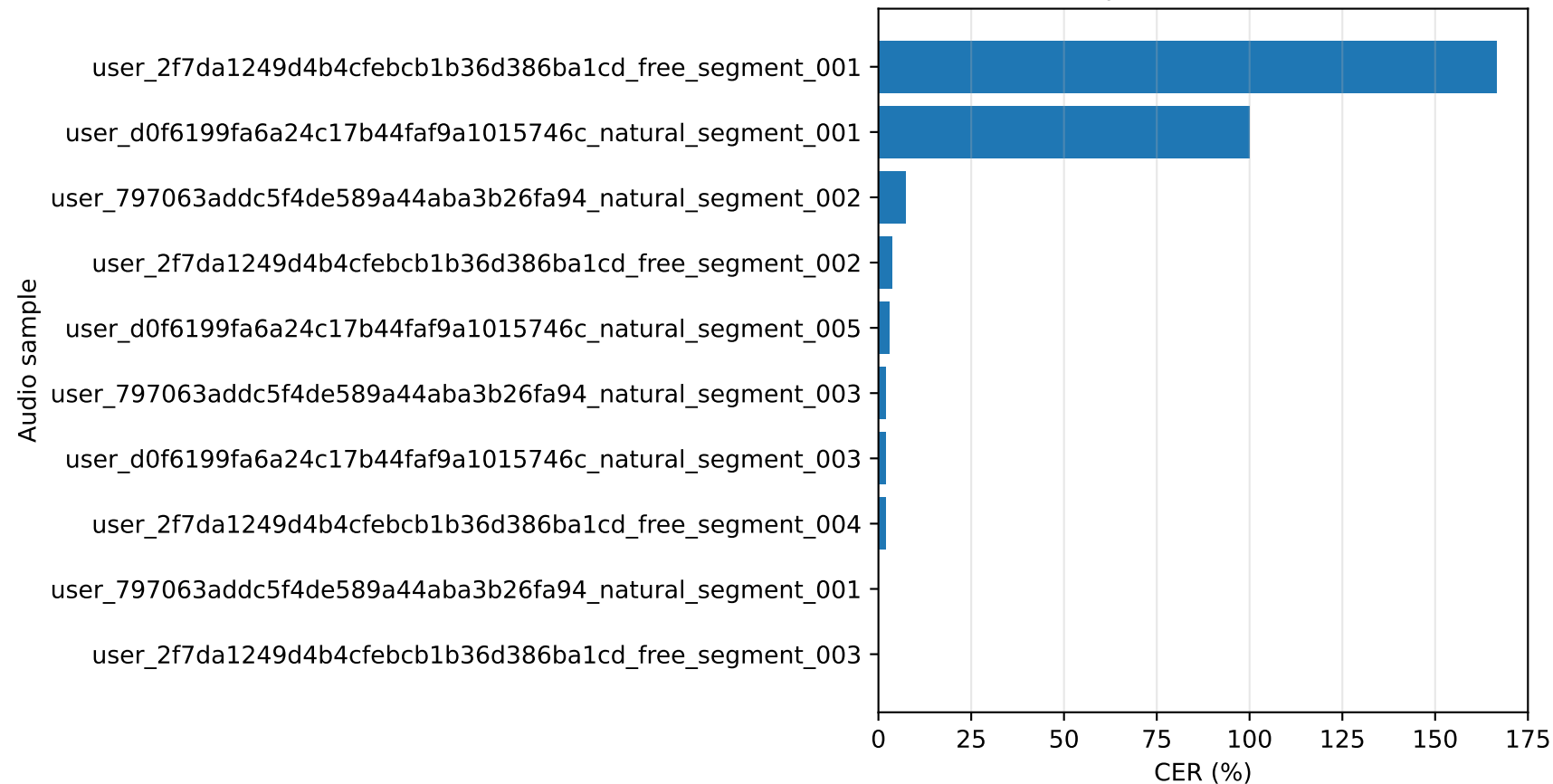
Hardest labeled samples for the default content model
