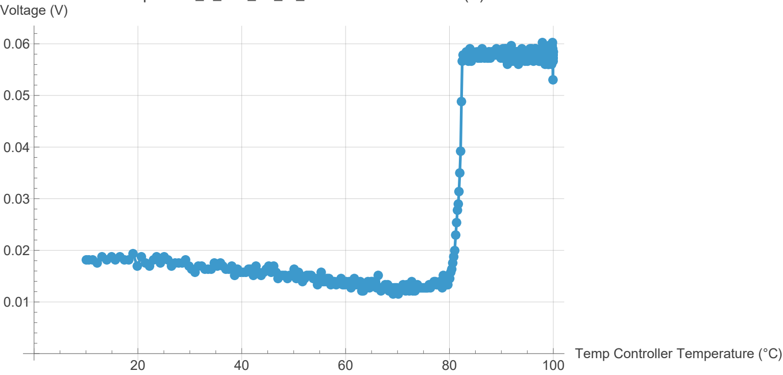
monoplmatin_0_rise_10_to_100.csv -- Channel3 (V)
