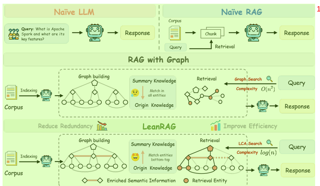
Figure 1: Comparison of typical LLM retrieval-augmented generation frameworks.
