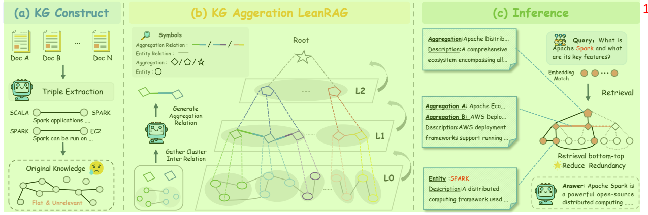
Figure 2: Overview of the LeanRAG framework.
