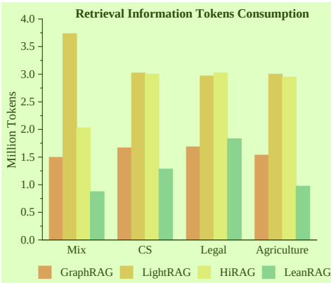
Figure 3: Comparison in retrieval tokens across four datasets
