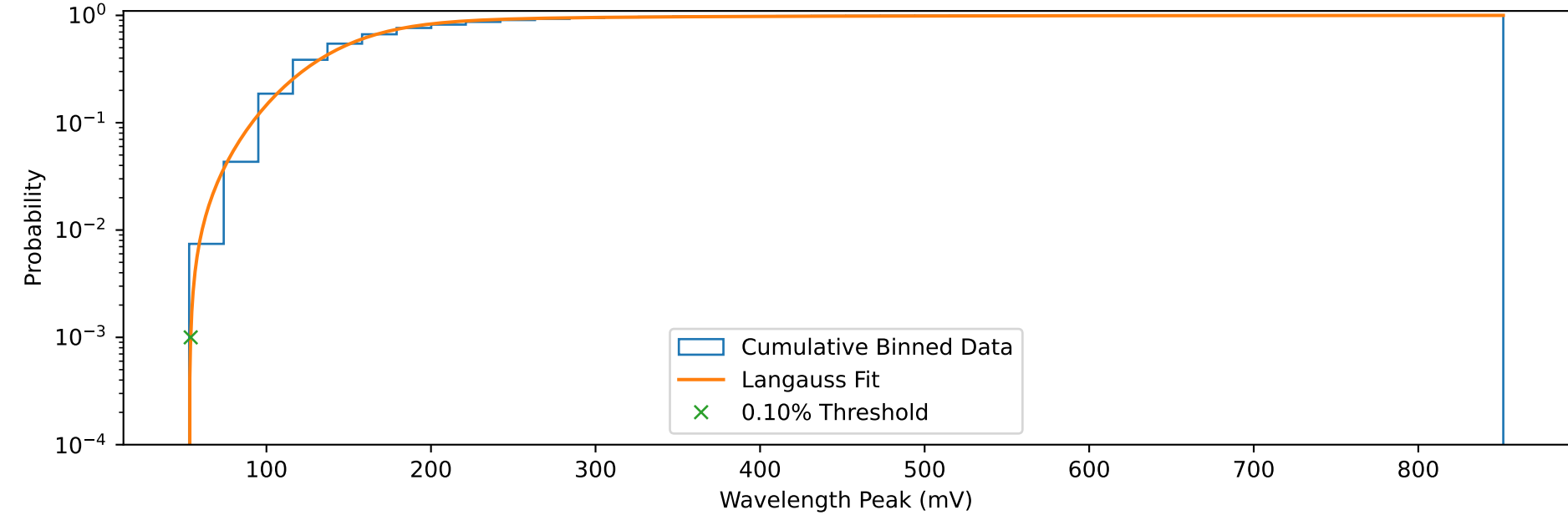
Distribution of Waveform Peaks
