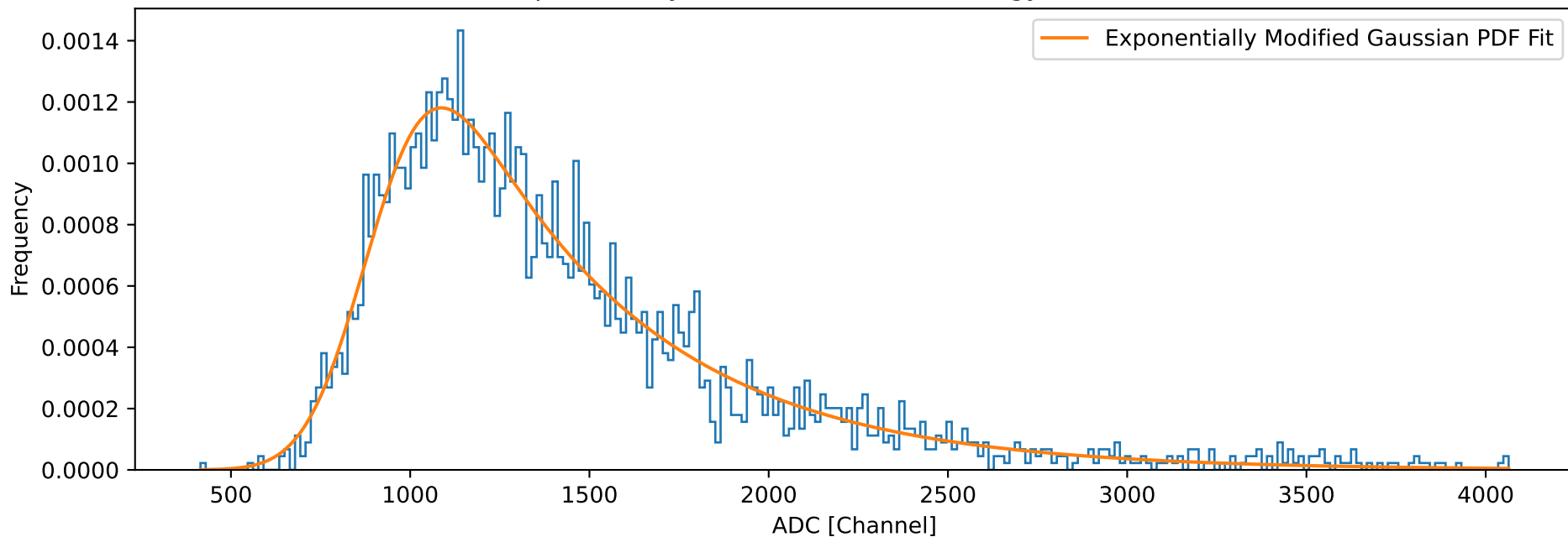
Exponentially Modified Gaussian Energy (Channel 1)
