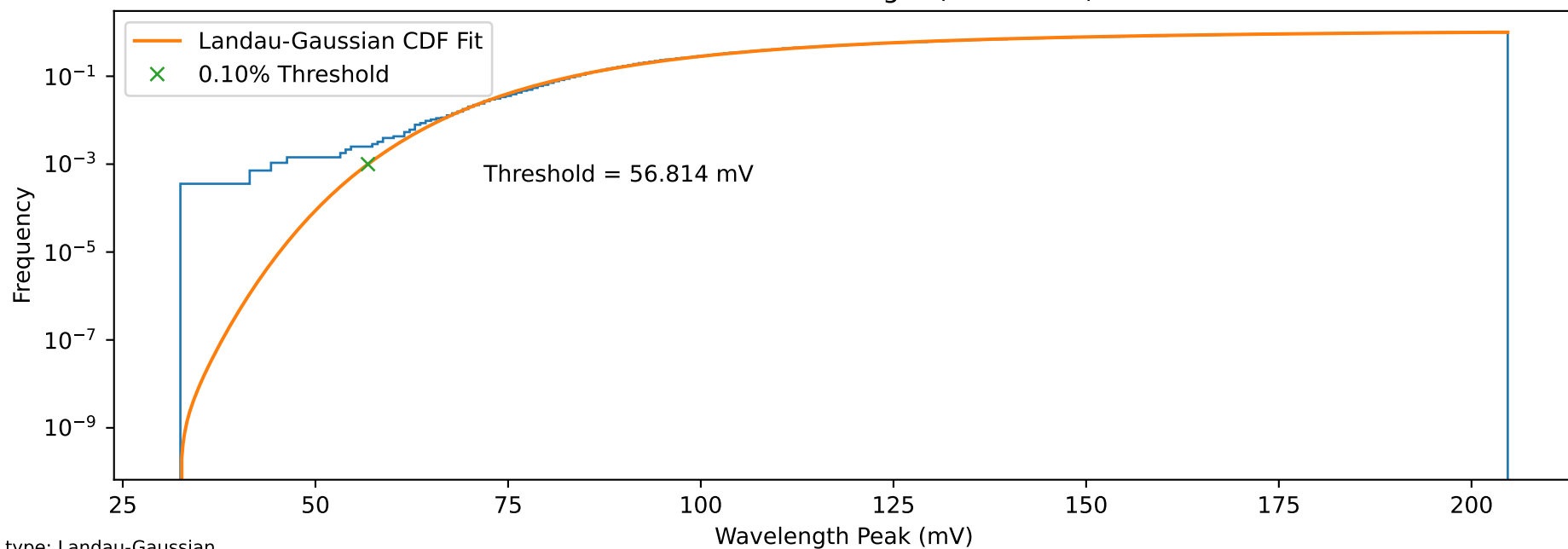
Landau-Gaussian Height (Channel 2)
