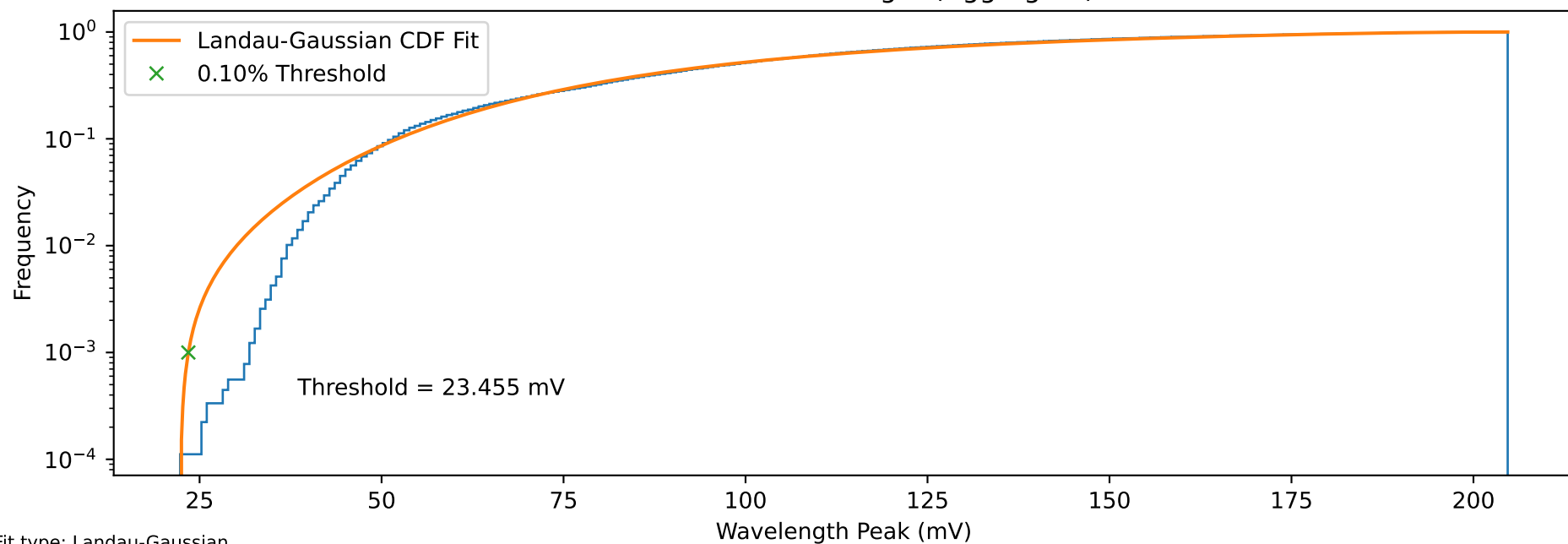
Landau-Gaussian Height (Aggregate)
