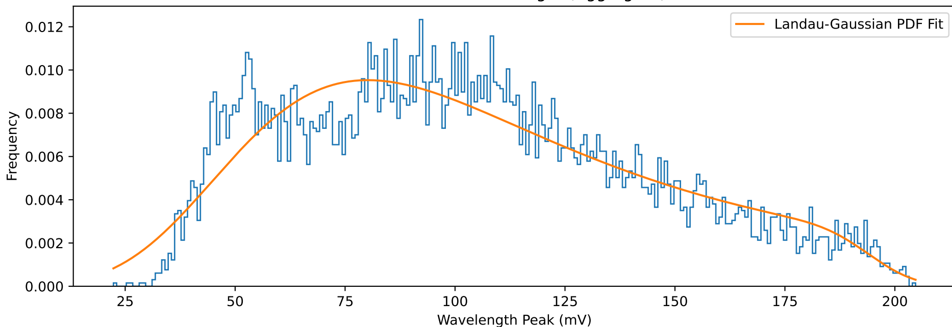
Landau-Gaussian Height (Aggregate)
