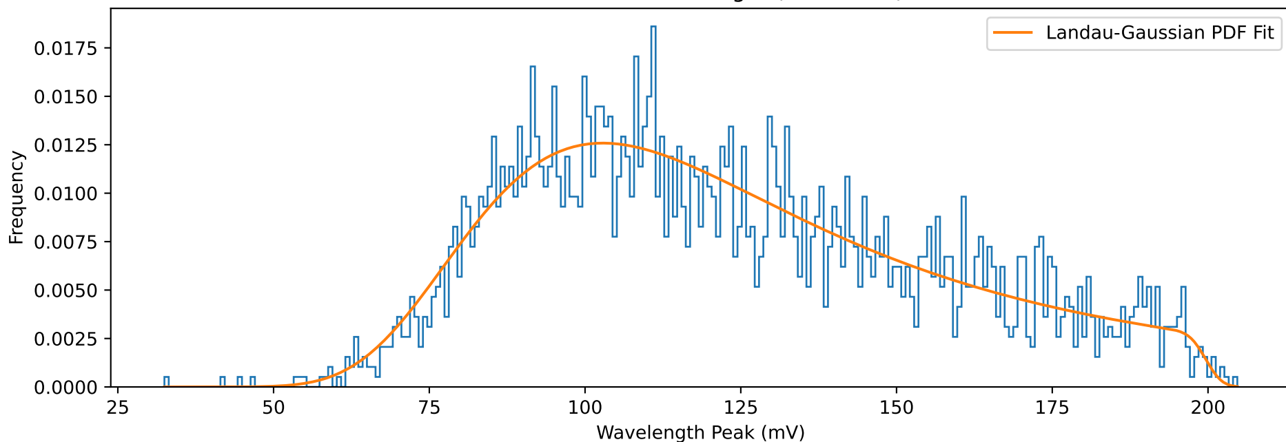
Landau-Gaussian Height (Channel 2)
