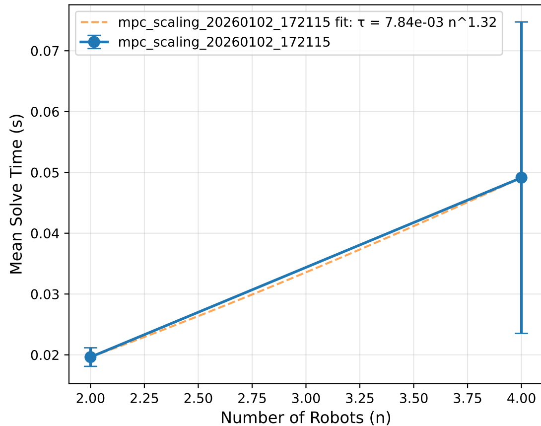
MPC Solve Time vs Team Size
