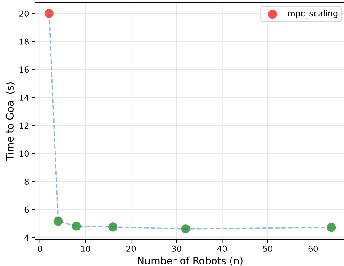
Convergence Time vs Team Size
