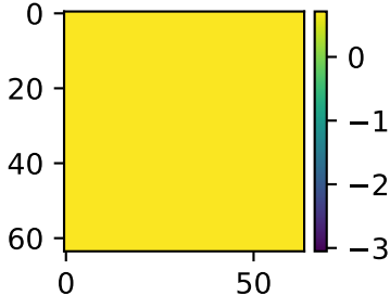
Pred.
