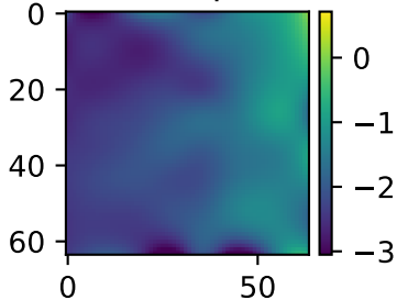
Interp.
