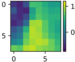
LR data
