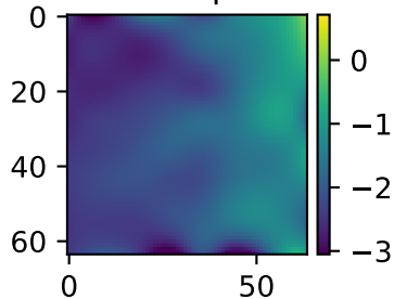
Interp.
