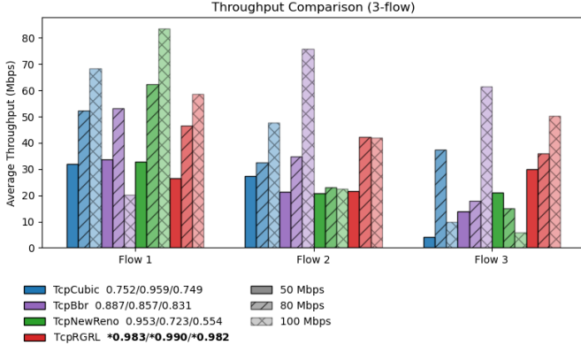
Fig. 5: Throughput comparison under different bottleneck bandwidths.
