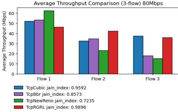
(b) Bottleneck bandwidth = 80 Mbps
