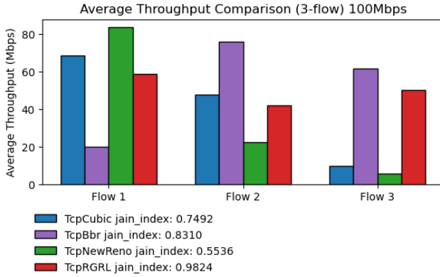
(c) Bottleneck bandwidth = 100 Mbps
