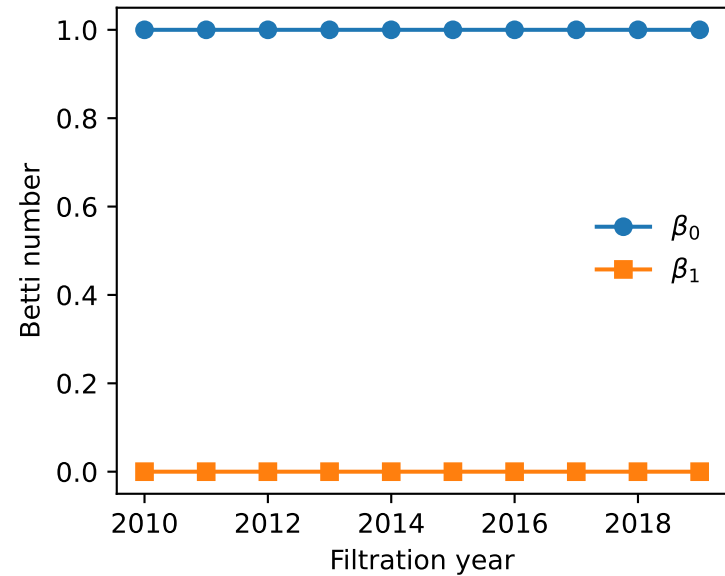
Betti curves
