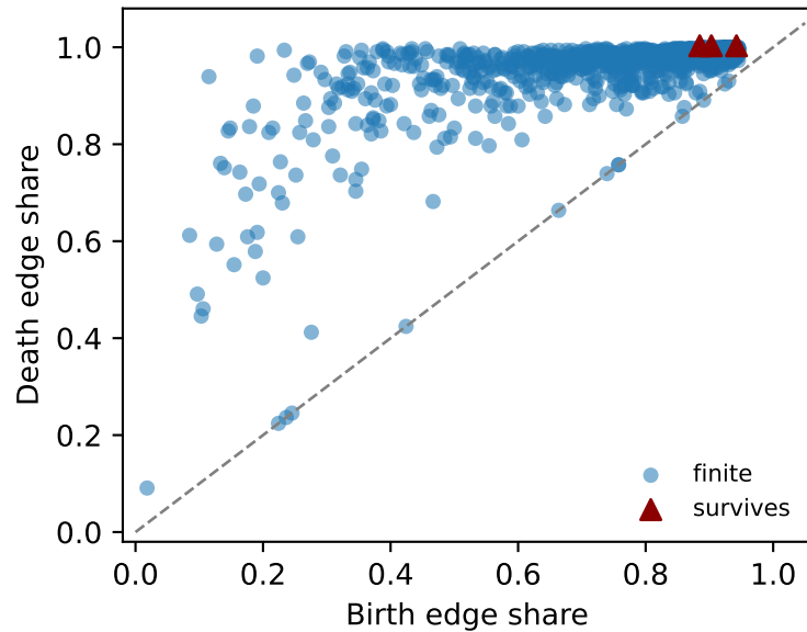
H_1 persistence diagram
