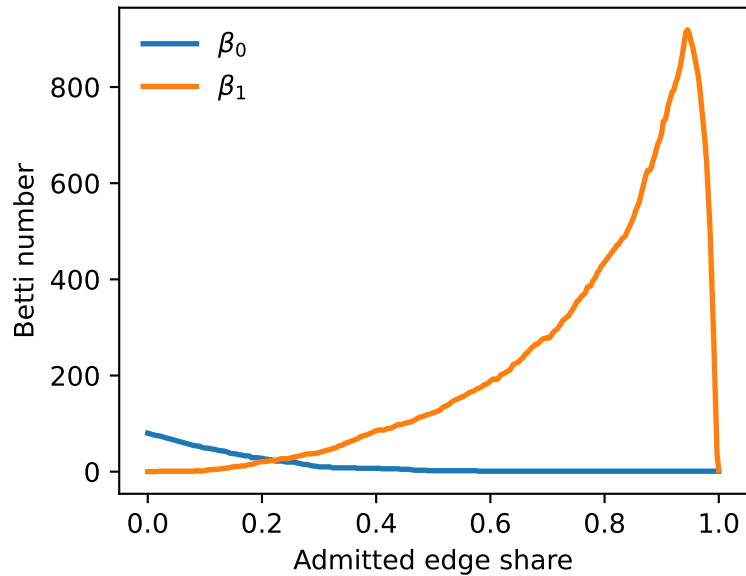
Betti curves: strong to weak ties
