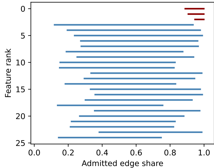
Longest H_1 barcode
