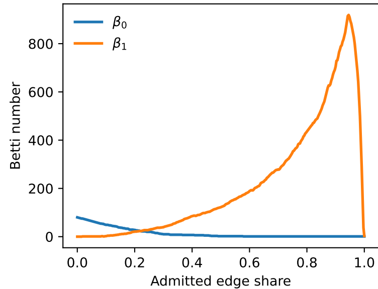
Betti curves: strong to weak ties
