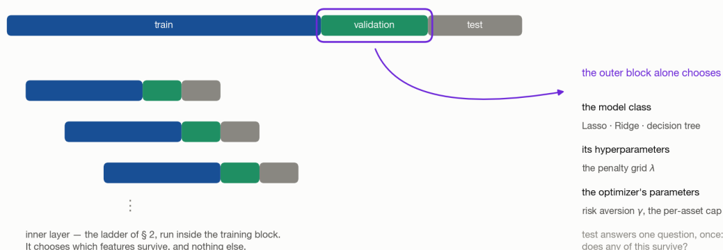
Figure 05.3: The two layers. The inner layer is the miniature ladder inside the training block, which chooses which features survive; the outer layer is the ringed held-out validation block, which chooses the model class, its hyperparameters, and the optimizer's parameters.
