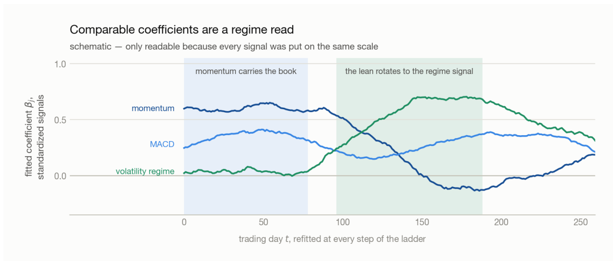
Figure 05.5: Three coefficient paths over a year of refits: momentum decays from high toward zero, a volatility-regime signal rises from zero to become the largest, and MACD stays between them. The shaded stretches mark where momentum carries the book and where the lean rotates to the regime signal.
