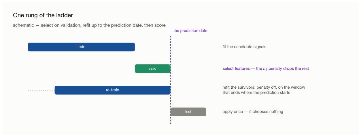
Figure 05.2: One iteration, in four stages: fit on train; select features on the validation segment; refit the survivors on a window shifted forward so that it ends where the prediction starts; apply once to test, beyond the dashed prediction date.
