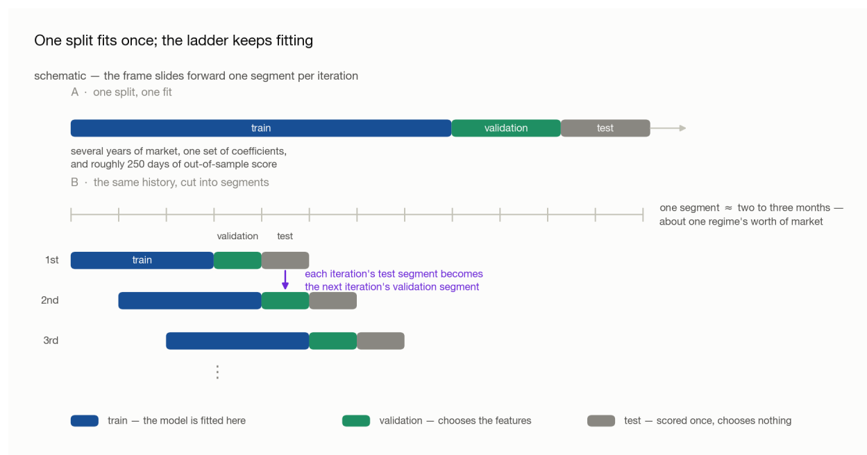
Figure 05.1: One split against the walk-forward ladder. Above, a single timeline cut once into train, validation and test. Below, the same history divided into twelve equal segments, with the train–validation–test frame starting one segment later on each row—so each row’s test segment is the next row’s validation segment.
